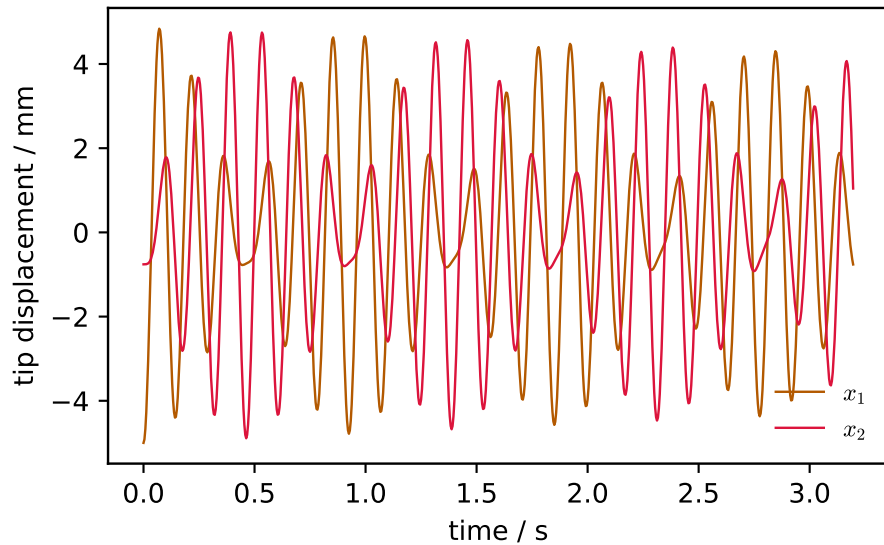
release at d = 24.5 mm: raw traces ( f_1 = 6.49 , f_2 = 7.56 Hz)
