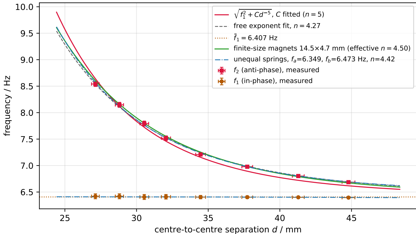
Graph 1: normal-mode frequencies against separation
