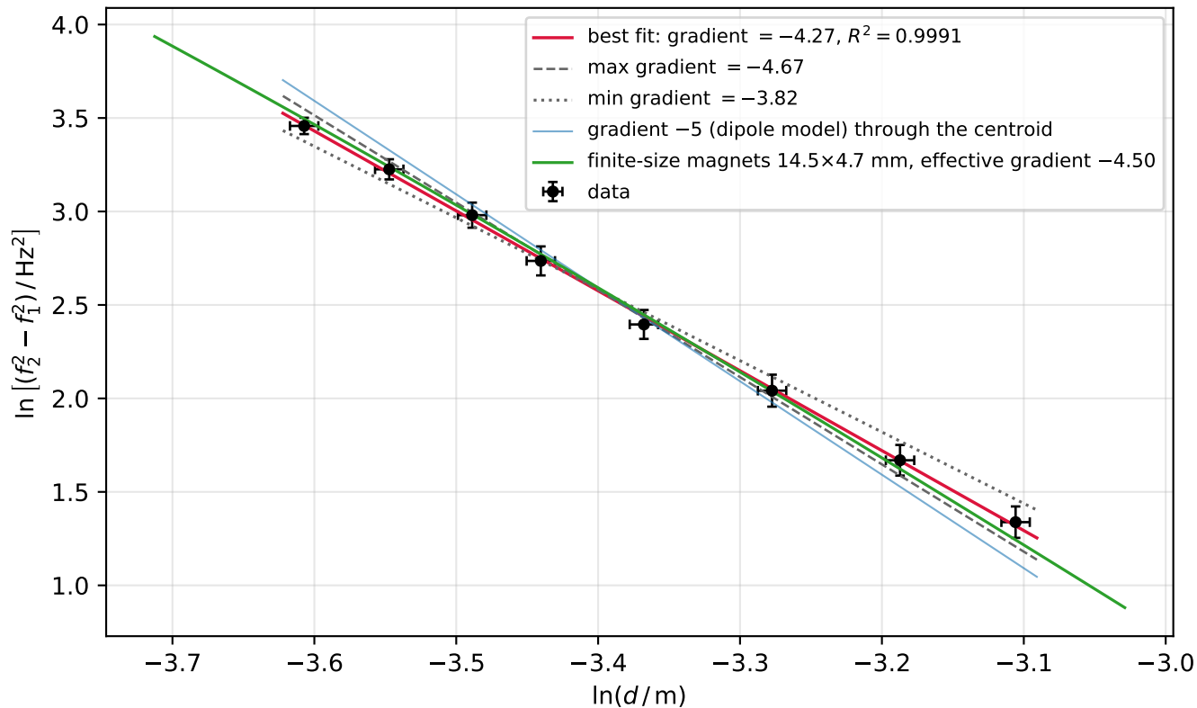
Graph 2: n = 4.27 \pm 0.42 (max/min gradient method)
