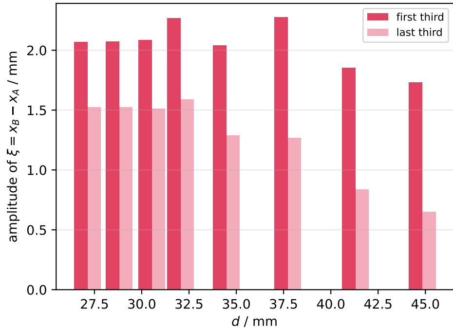
Graph 10b: anti-phase amplitude (change of separation)
