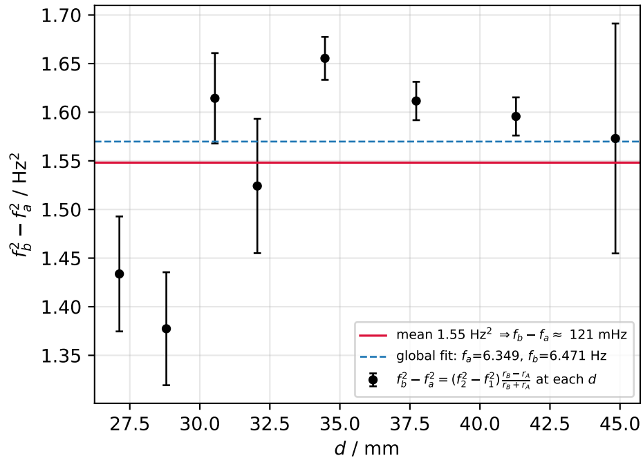
Graph 9a: spring detuning from r_A vs r_B (should be the same at every d )
