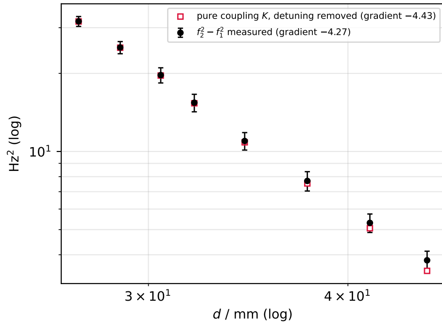
Graph 9b: detuning does not change the exponent
