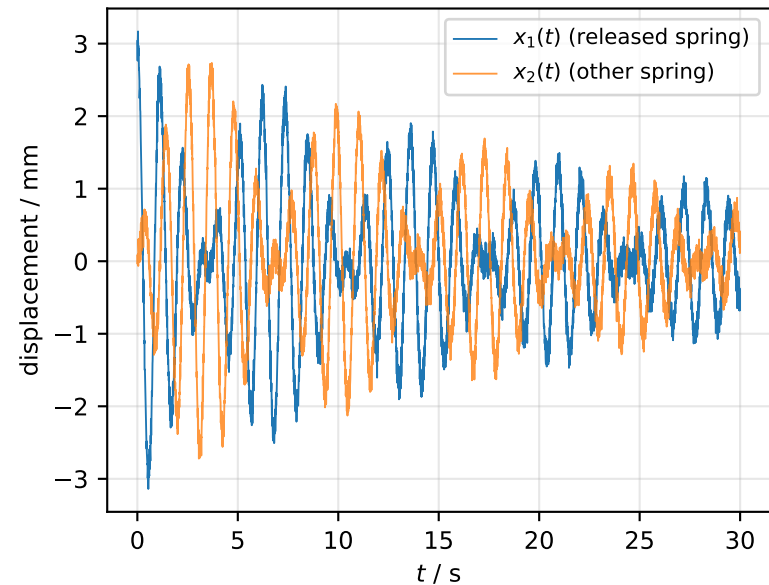
beats: energy moves back and forth between the springs
