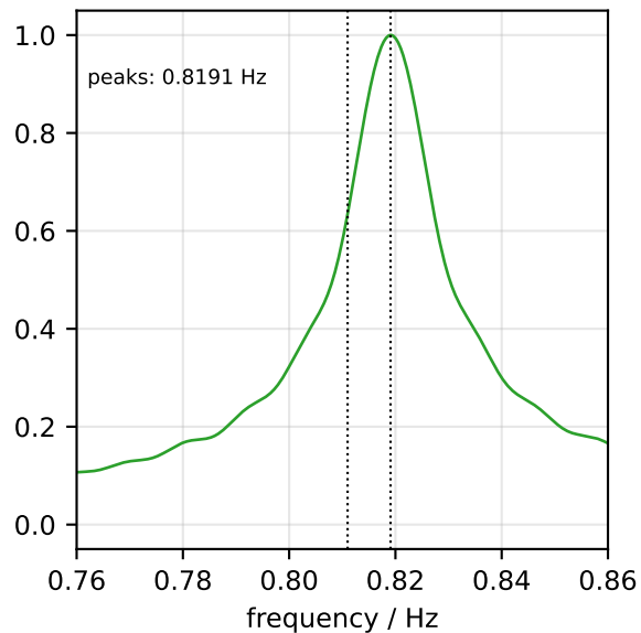
FFT of \xi = x_1 - x_2
