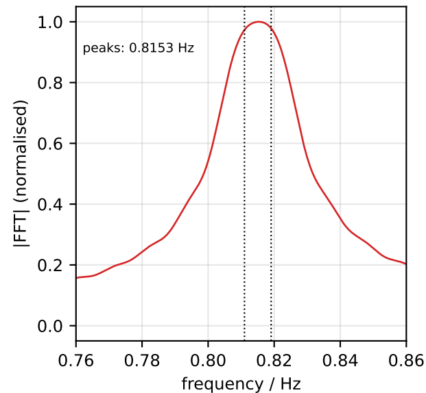
FFT of x_1 alone
