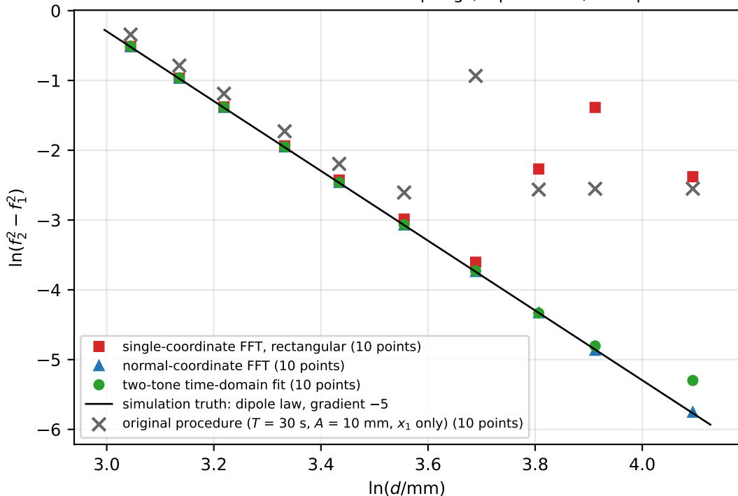
SIMULATED records: identical springs, dipole force, 240 fps
