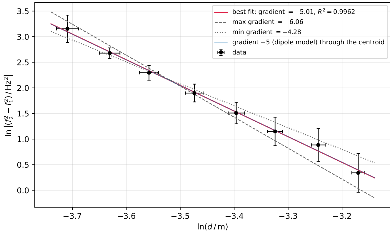
Graph 2: n = 5.01 \pm 0.89 (max/min gradient method)
