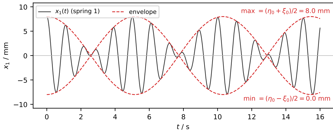
(a) ideal instantaneous release: x_1(0) = A , x_2(0) = 0
