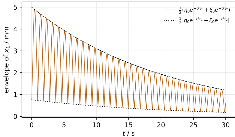
(a) equal decay times (internal friction, air): minima/maxima stay = x_{20}/A
