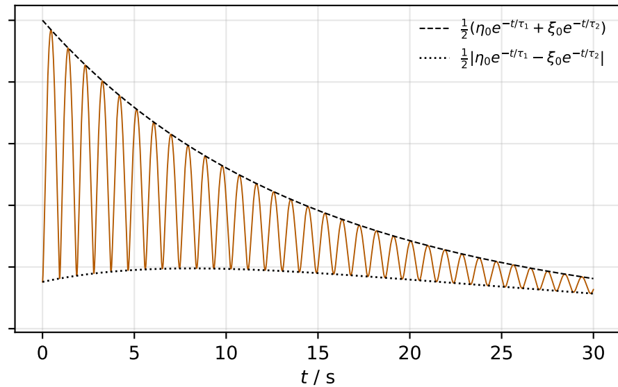
(b) anti-phase mode decaying twice as fast (e.g. eddy currents)
