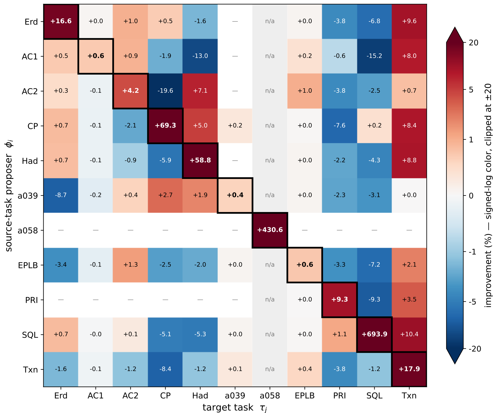
In-task adaptation gains vs. zero-shot cross-task transfer diagonal: full Weight vs. Initial | off-diagonal: Best@6 vs. untrained proposer
