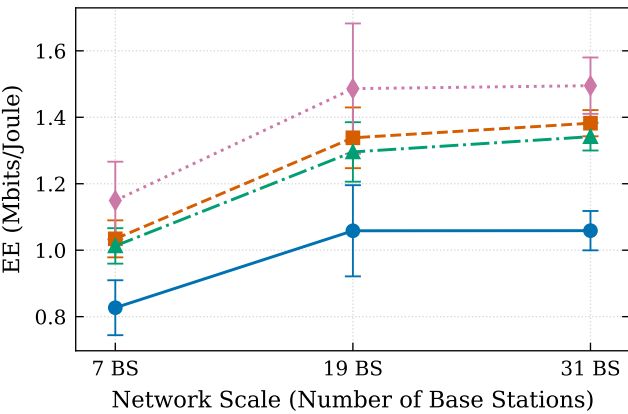
(c) Network Energy Efficiency
