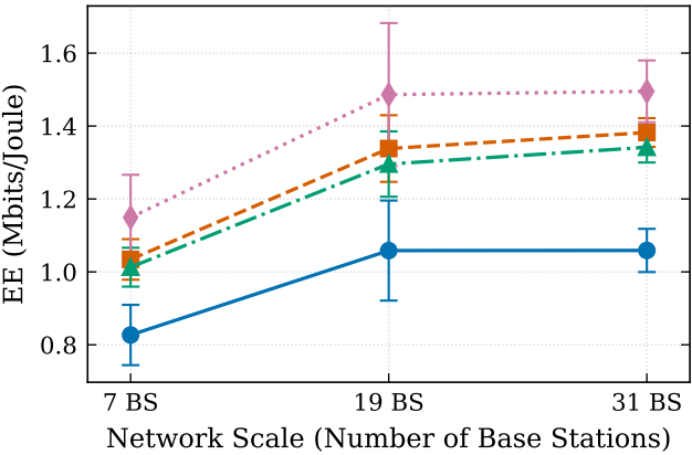
(c) Network Energy Efficiency
