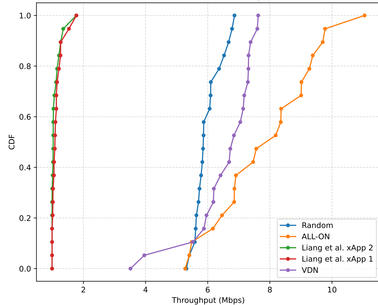
CDF: 10th Percentile Throughput
