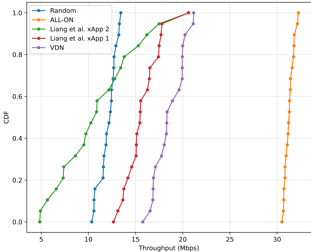
CDF: Average Throughput
