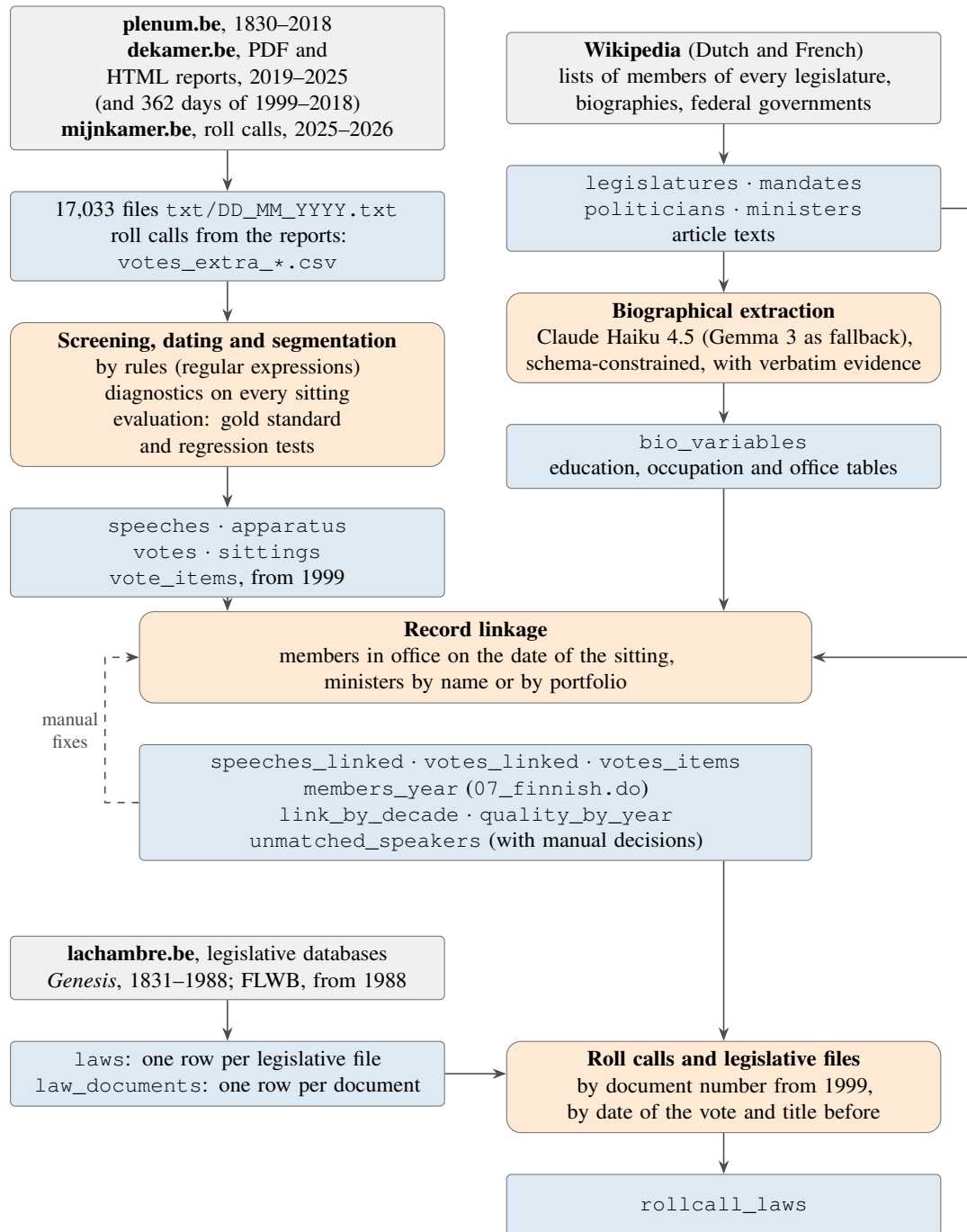
Fig. S1. Construction of the dataset. Grey: sources; blue: files released with the dataset (CSV unless stated otherwise); orange: processing steps. The debates (left) and the registers of members and ministers (right) are built independently and joined by date-aware record linkage; the legislative files (bottom) are read from the Chamber’s legislative databases and joined to the roll calls by document number or by the date of the vote and the title. Names that cannot be linked automatically are resolved by hand in unmatched_speakers.csv , and these decisions are released with the data. The Senate module (1880–1914) goes through the same steps.
