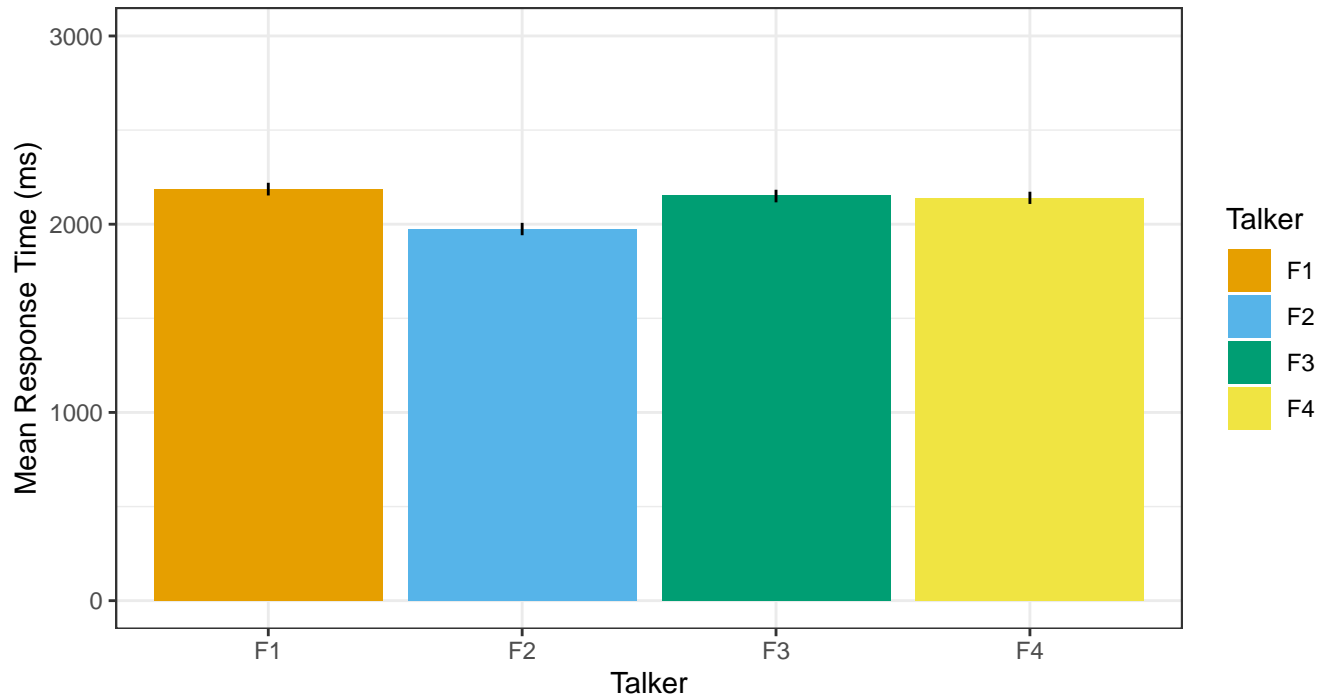
Mean Sharp/Dull Response Times by Talker
