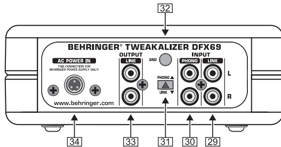
Fig. 2.2: The rear panel connections
