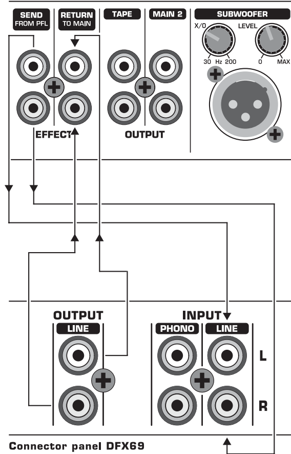
Fig. 3.1: Connecting to the effects loop of the PRO MIXER VMX1000
