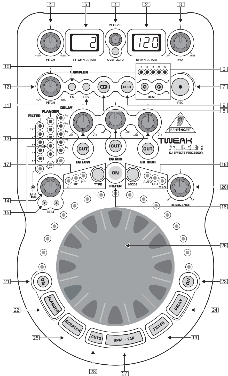
Fig. 2.1: DFX69 control elements
