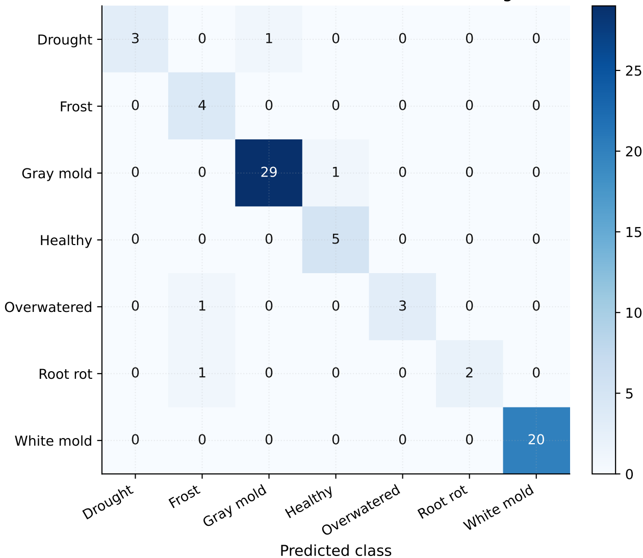
ResNet v2 confusion matrix on the clean 70-image holdout
