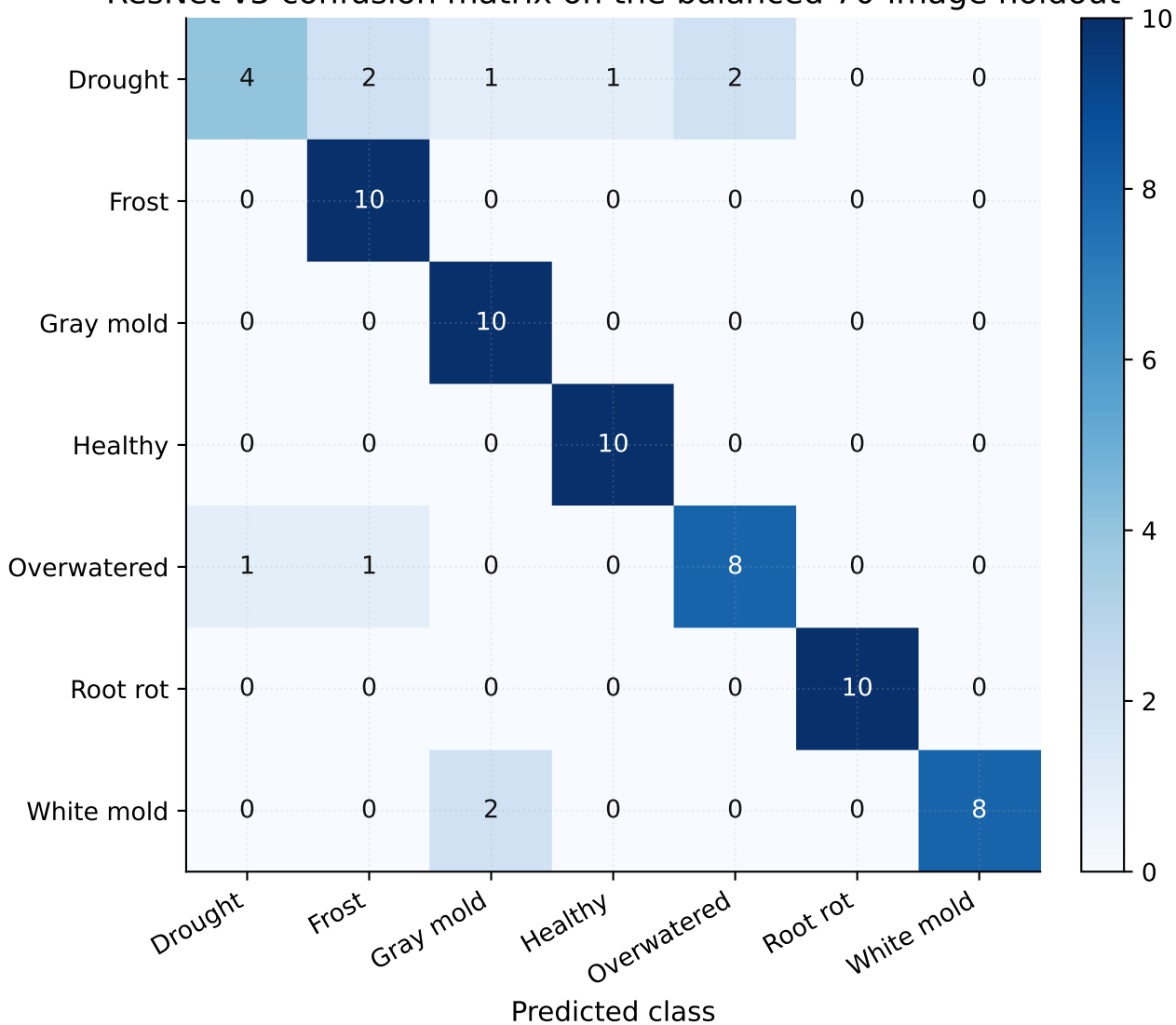
ResNet v3 confusion matrix on the balanced 70-image holdout
