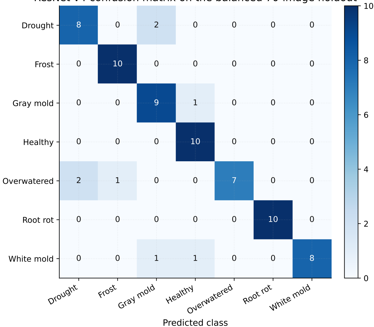
ResNet v4 confusion matrix on the balanced 70-image holdout
