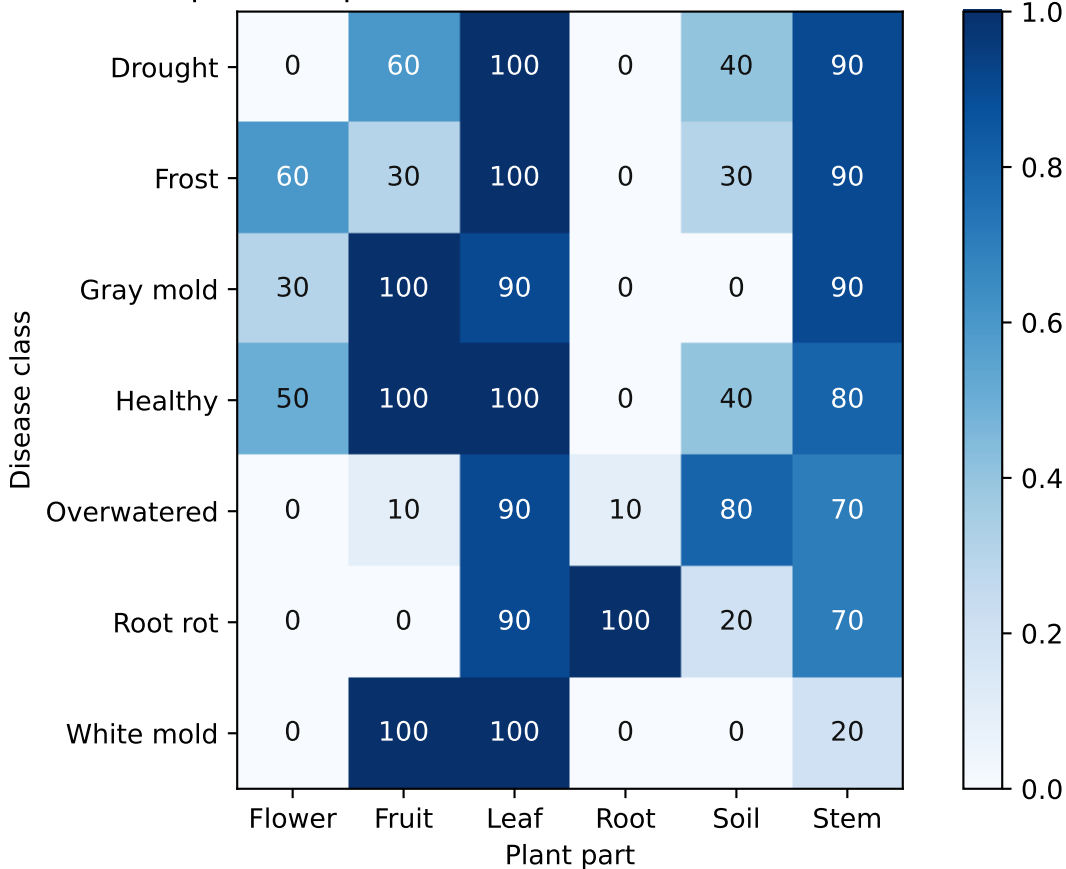
RF-DETR per-class part-detection rate on the disease holdout (\%)
