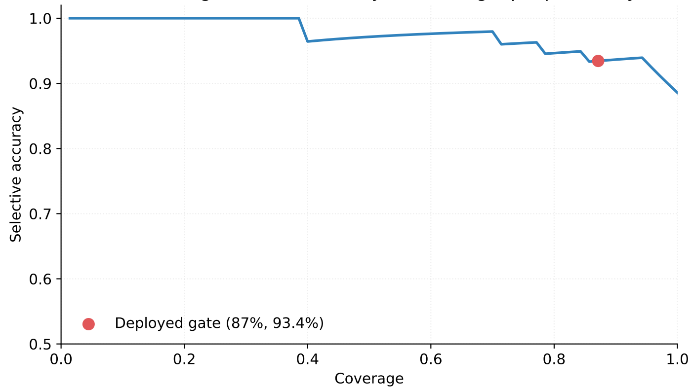
Risk-coverage curve, ordered by descending top-1 probability
