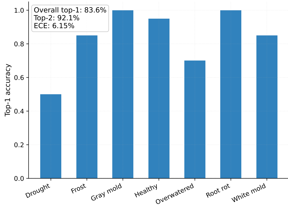
Per-class top-1 accuracy on the balanced holdout
