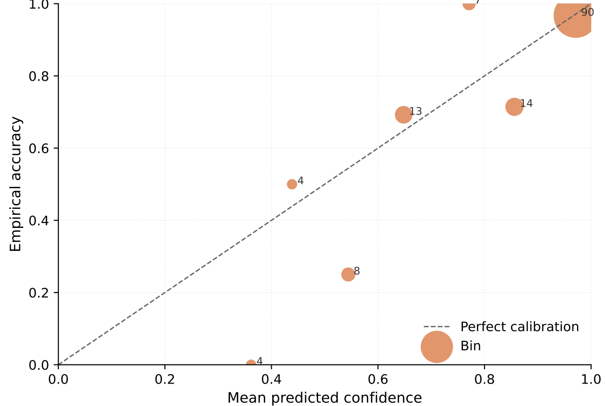
V3 reliability diagram, ECE = 6.15%
