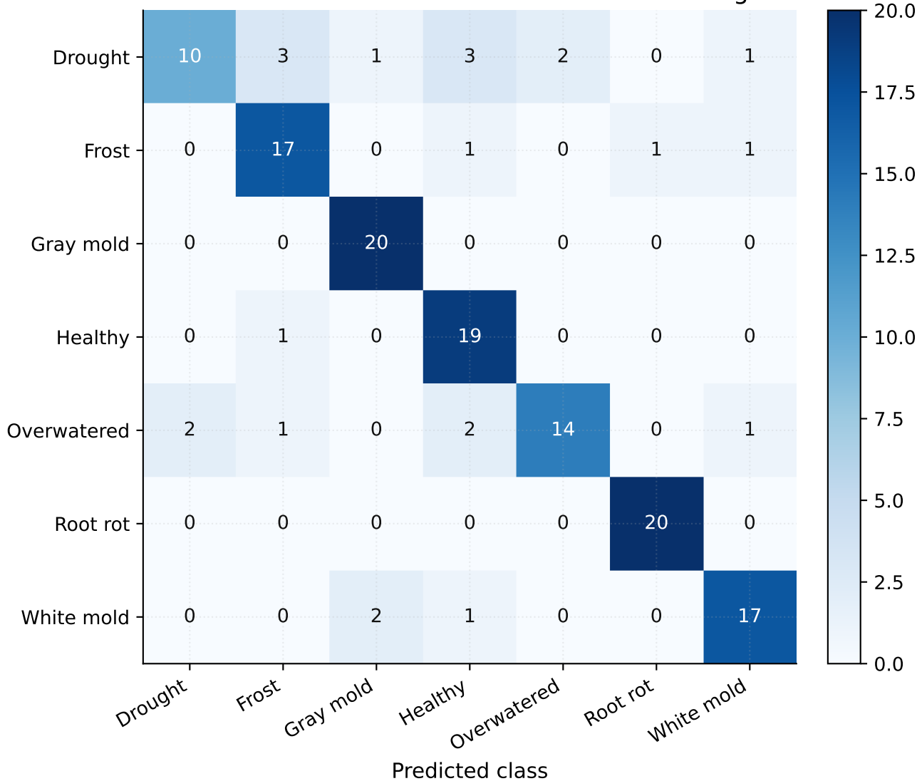
ResNet v3 confusion matrix on the balanced 140-image holdout
