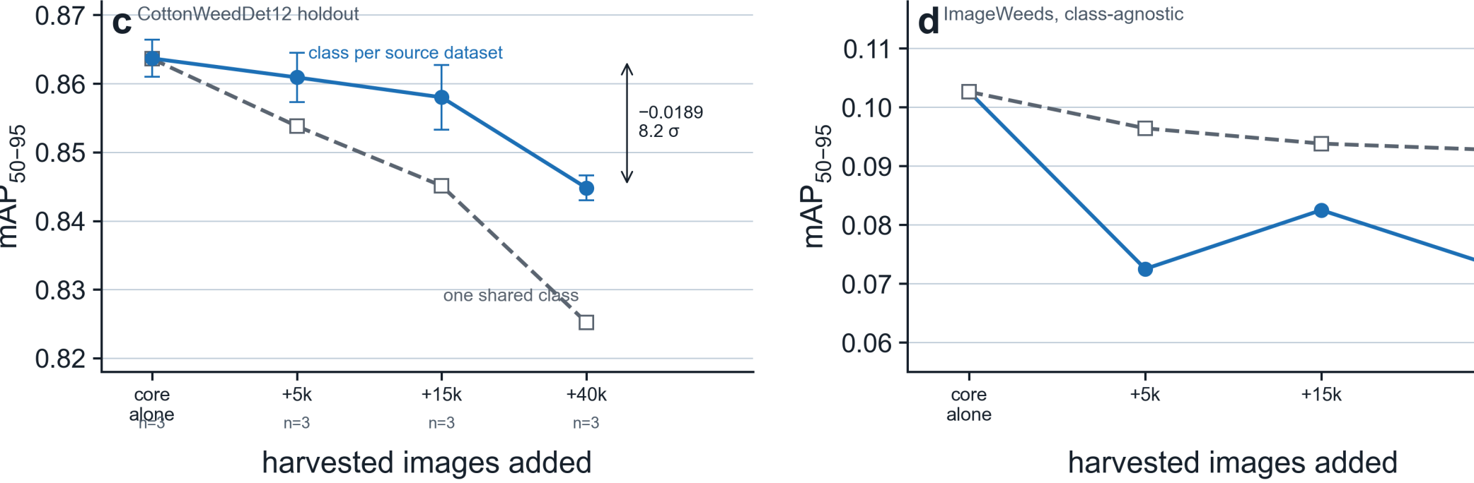
Figure 4. (c) Three seeds at every rung on our own sealed holdout. (d) The same eight checkpoints on a second weed dataset they never saw. Both exams fall, so the narrow metric is not what makes the ladder drop.
