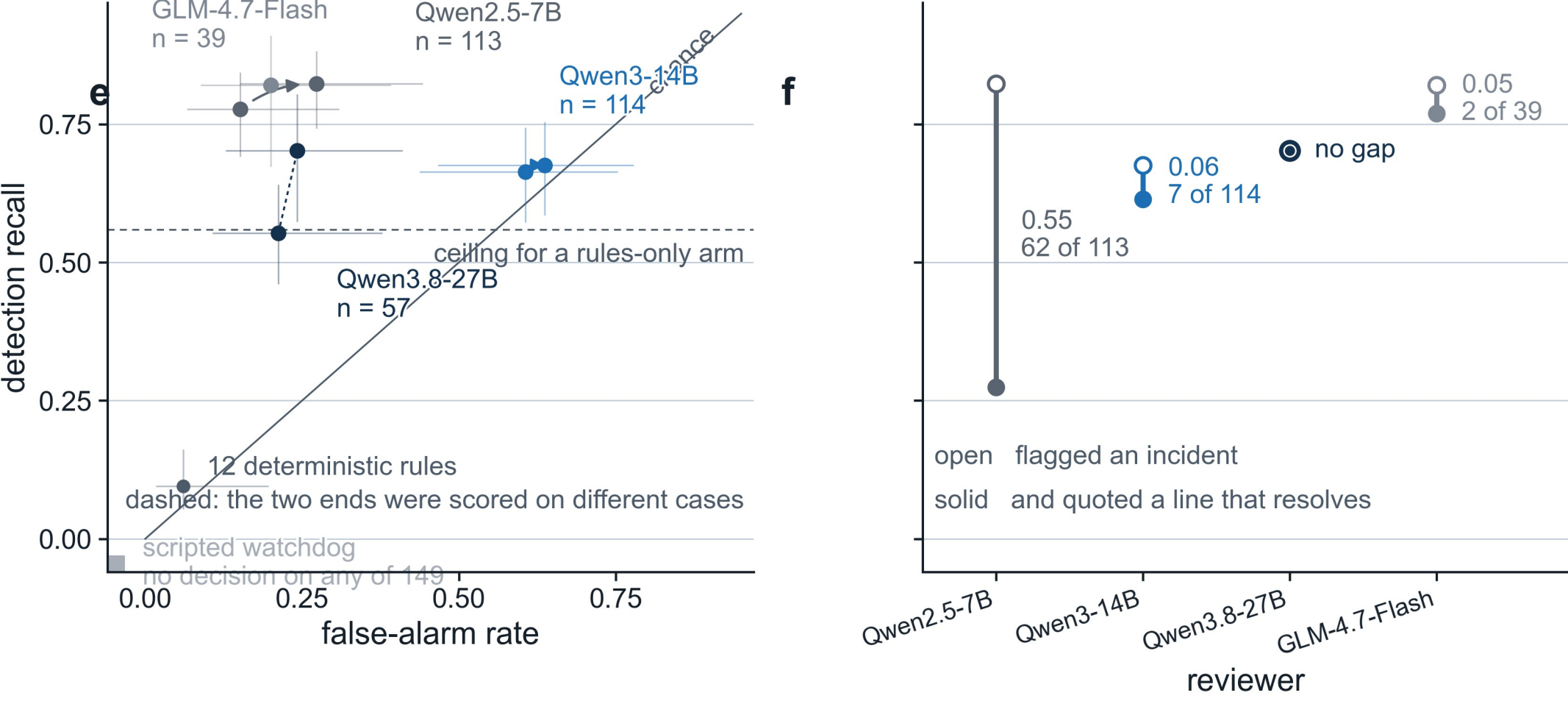
Figure 3. (e) Recall and (f) grounded recall on one frozen corpus of real incidents from this project's own record, scored by the project's own scorer. Each mark carries its own denominator and bars are 95% Wilson intervals. The 7 B has the highest recall on the page and 0.55 of it quotes nothing; the 27 B has no such gap.
