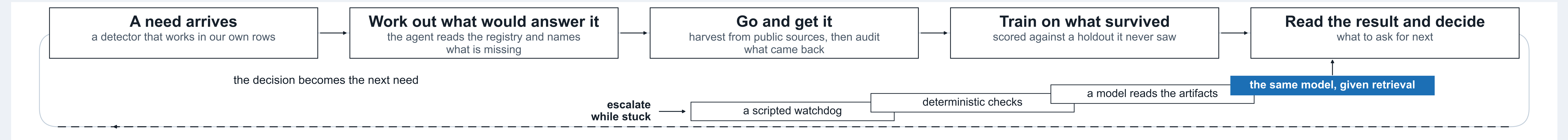
Figure 2. A need arrives, the agent works out what data would answer it, fetches it, trains on what survives the audit, scores, decides what to ask next. Stuck, it climbs the ladder. Dashed: the decision is recorded, nothing reads it back.
