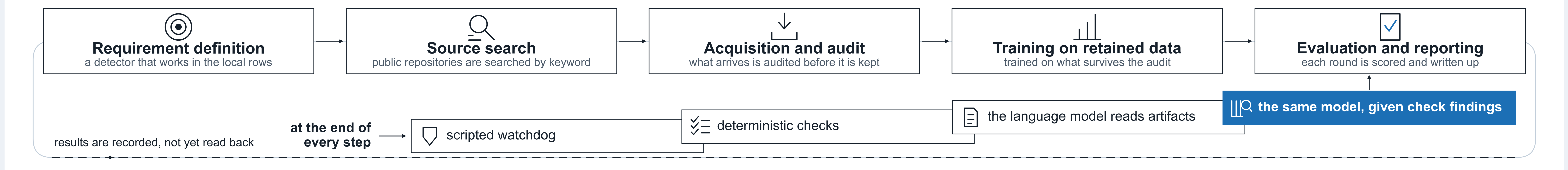
Figure 1. The loop an agent runs unattended. A requirement is turned into keyword queries, what they return is audited, what survives is trained on, and the round is scored. The pictures that score the model also choose which epoch is reported. Review follows every step, not only when something looks wrong, and the return edge is dashed because nothing reads the decision back yet.
