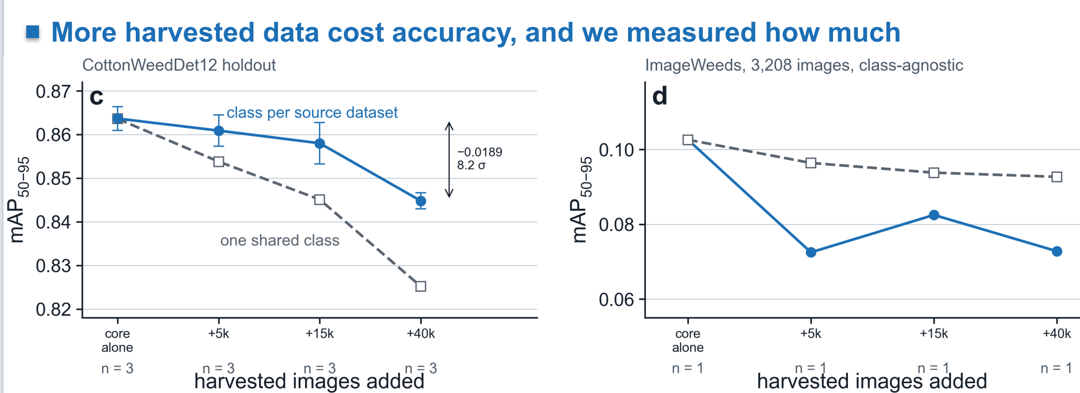
Figure 4. (c) Three seeds at every rung on our own sealed holdout, marks are the mean with 1 s.d. (d) The same eight checkpoints on a second weed dataset they never saw, one seed per rung. Both exams fall. Starting fresh instead of from the last round's weights recovers +0.0287, 5.1 times this recipe's seed spread. That is the change the next campaign makes.
