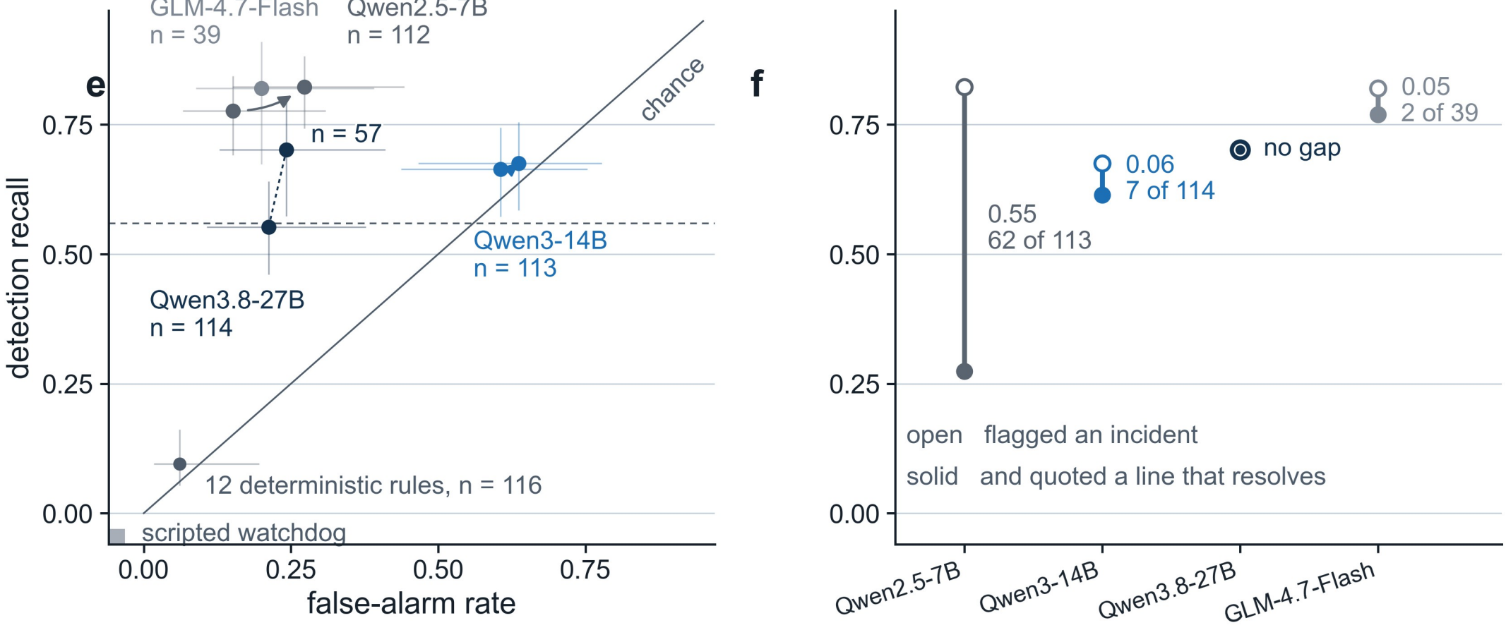
Figure 2. (e) Recall and (f) grounded recall on 149 frozen failures taken from this project's own record, scored by the project's own scorer. Each arrow runs from the model reading the raw files to the same model handed the twelve checks' findings. Grounded counts only the cases where the model also quoted a line that resolves the failure. The dotted arrow carries no head: its two ends were scored on different cases, 57 against 114.
