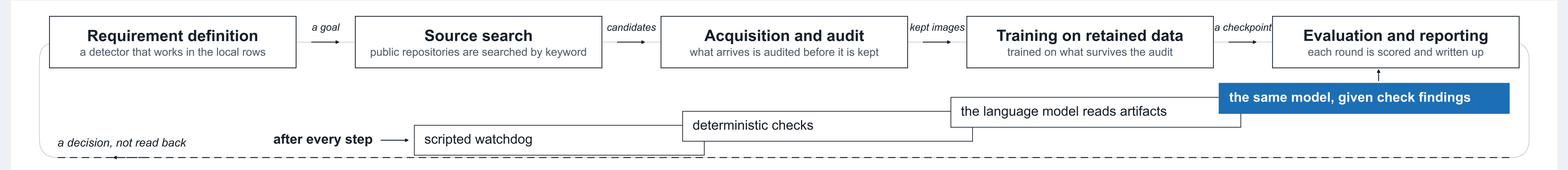
Figure 1. The loop an agent runs unattended, with the object each step hands to the next. A requirement is turned into keyword queries, what they return is audited, what survives is trained on, and the round is scored. The pictures that score the model also choose which epoch is reported. Review follows every step, climbing the tiers only while it is stuck, and the return edge is dashed because nothing reads the decision back yet.
