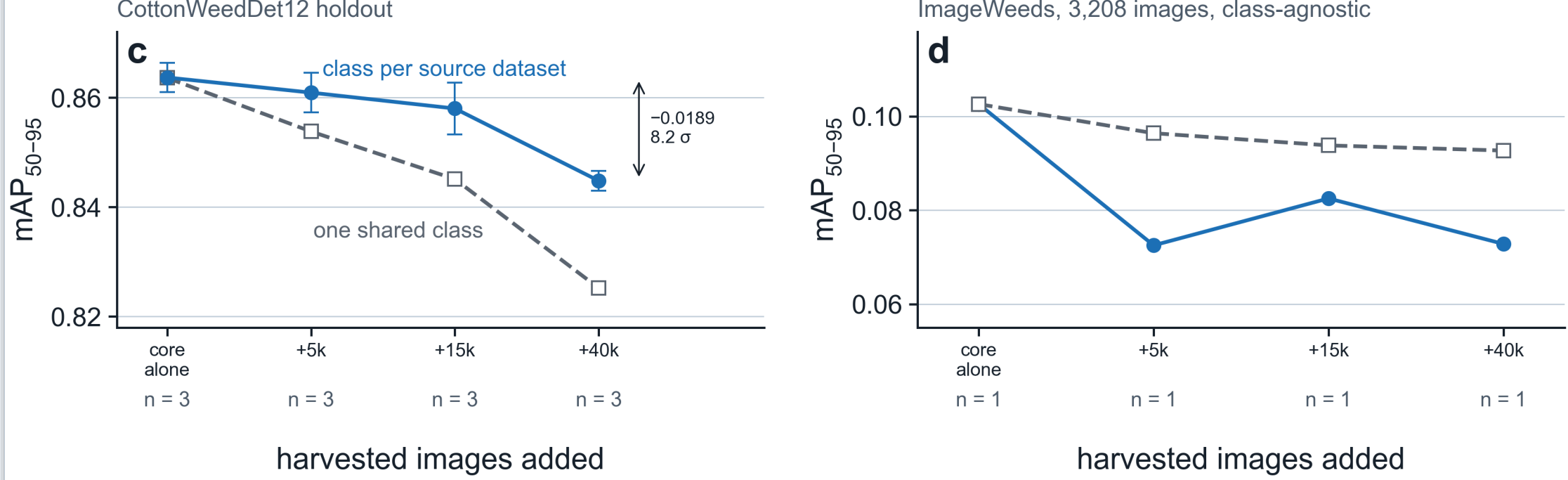
Figure 4. (c) Three seeds at each level, mean and 1 s.d., on the 1,977-image holdout, which is also each run's validation set, so every mark is that run's best epoch. (d) The same eight checkpoints on an unseen weed dataset, one seed per level. Both panels decline.
