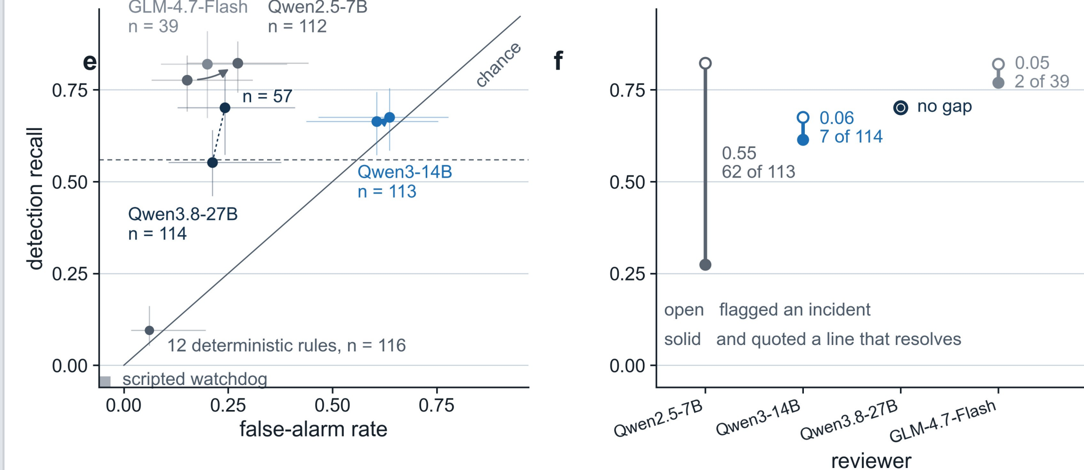
Figure 3. (e) Recall and (f) grounded recall on one frozen corpus of real incidents from this project's record, scored by its own scorer. Each tail is the language model on artifacts with the twelve checks' findings withheld; each head is the same model supplied with them. The dotted line has no arrowhead: its ends were scored on different cases, the 27 B head on 57 incidents and its tail on 114.
