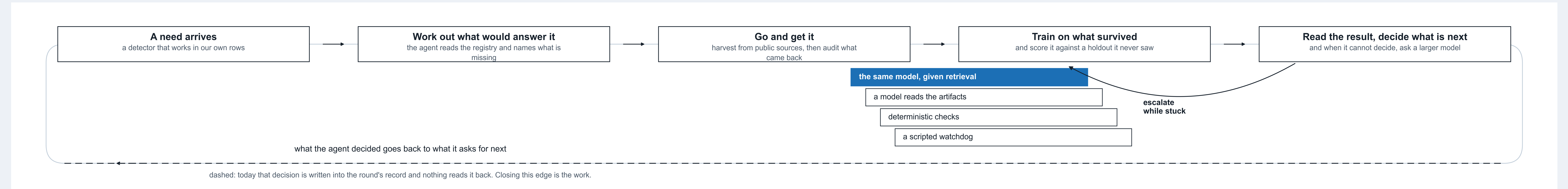
Figure 2. The loop an agent runs to answer a need, drawn as a loop. A need arrives, the agent works out what data would answer it, goes and gets it, trains on what survives the audit and scores it, then reads its own result and decides what to ask for next. When it cannot decide it climbs the ladder inside the loop, each rung reading the one below it and free to overrule it. The outward run is solid because it runs unattended today. The return run is dashed because it is the one edge the platform has not closed: the decision is recorded and nothing reads it back, and closing it is the work this poster is about.
