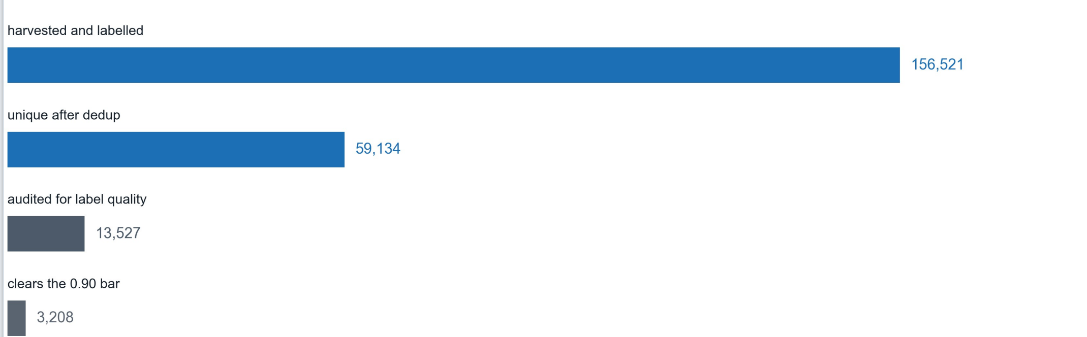
Figure 5. One of six audited harvested sources clears the label-precision bar. The audit probe reads 1.000 on human-labelled CottonWeedDet12, so the low scores are the data.
