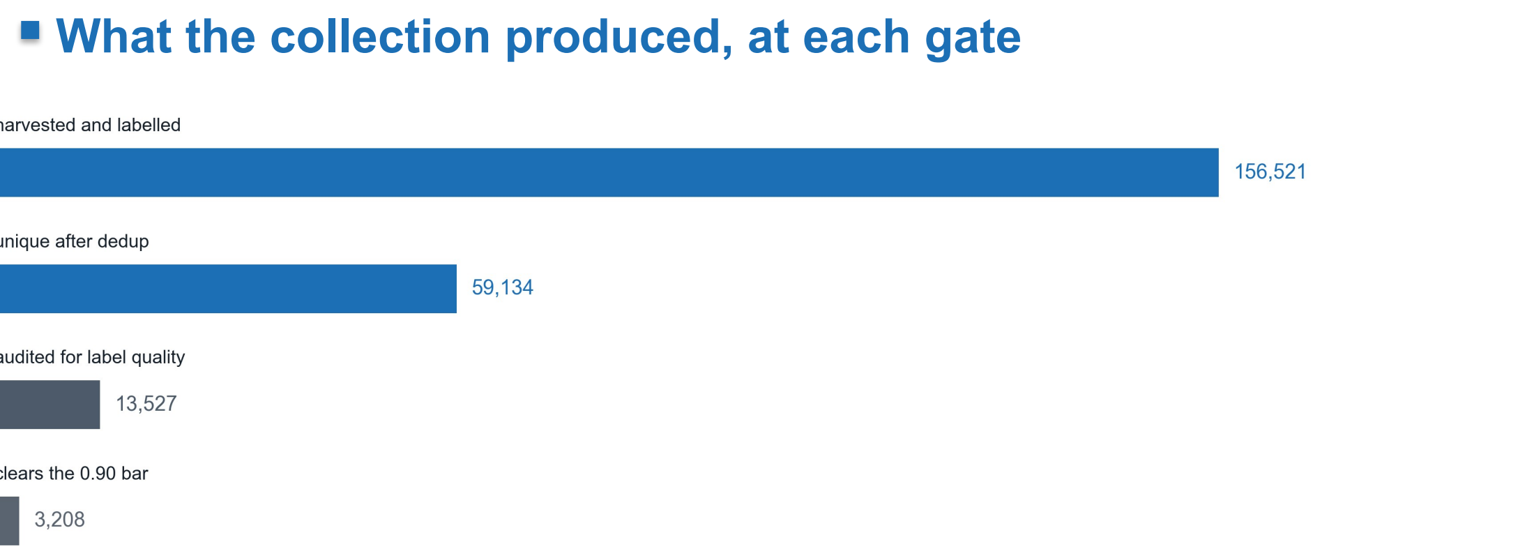
Figure 5. One of six audited harvested sources clears the label-precision bar. The audit probe reads 1.000 on human-labelled CottonWeedDet12, so the low scores are the data.
