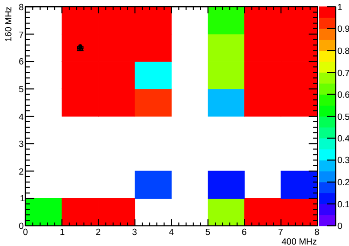
BPix_Bml_SEC3_LYR1_LDR2H_MOD2_nTBMDecodes
