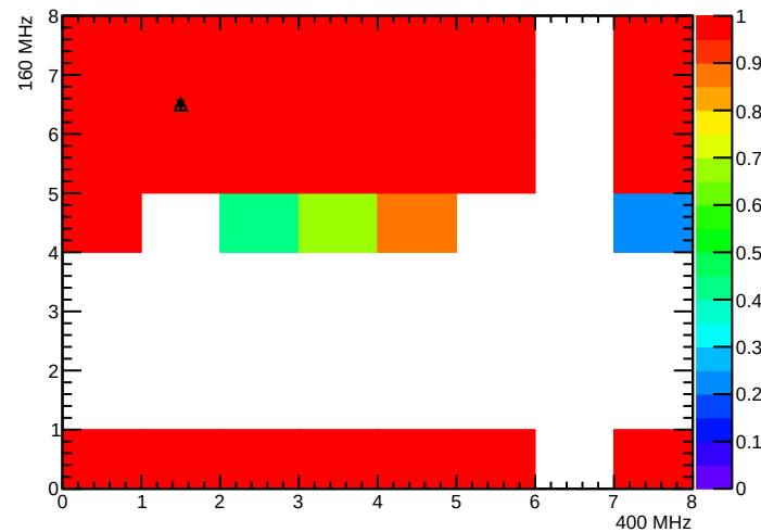
BPix_BmO_SEC5_LYR1_LDR4H_MOD2_nROCHheaders
