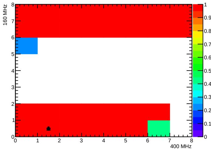
BPix_Bml_SEC5_LYR3_LDR13F_MOD2_nTBMDecodes
