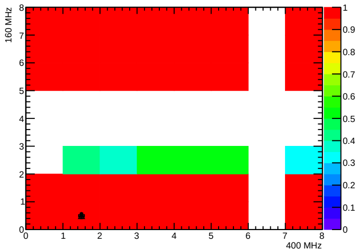
BPix_BpI_SEC4_LYR2_LDR7F_MOD3_nTBMDecodes
