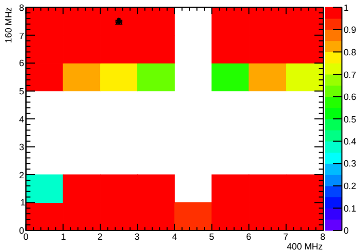
BPix_Bml_SEC5_LYR2_LDR9F_MOD4_nTBMDecodes
