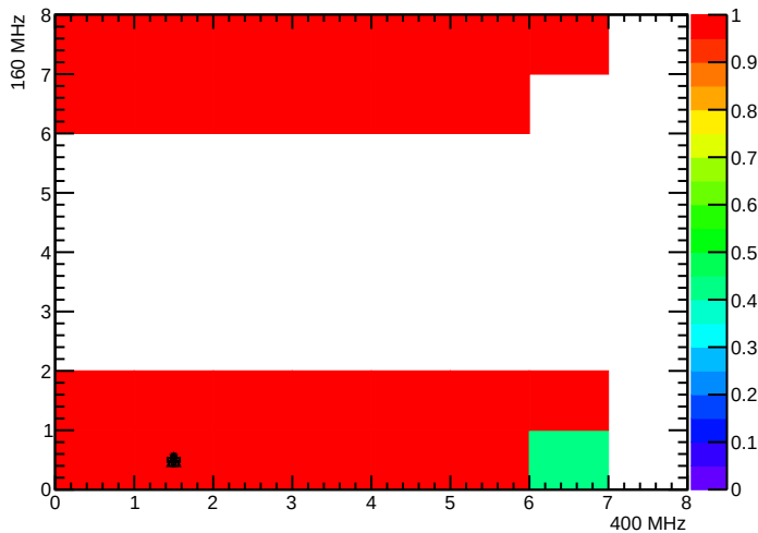
BPix_Bml_SEC6_LYR4_LDR23F_MOD1_nTBMDecodes
