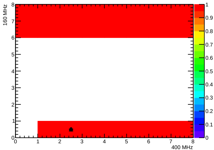
BPix_BpO_SEC4_LYR4_LDR15F_MOD4_nTBMDecodes
