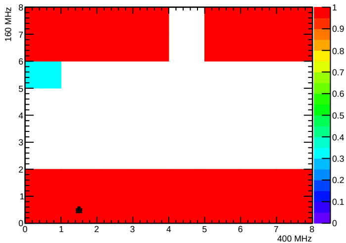
BPix_BpO_SEC7_LYR4_LDR28F_MOD1_nTBMDecodes
