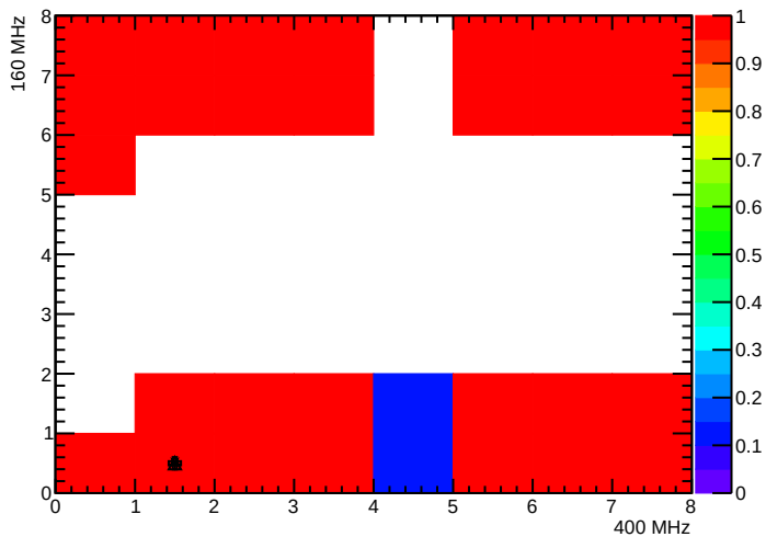
BPix_BpO_SEC2_LYR3_LDR5F_MOD3_nTBMDecodes
