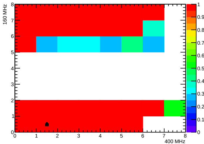
BPix_Bpl_SEC7_LYR2_LDR11F_MOD3_nTBMDecodes
