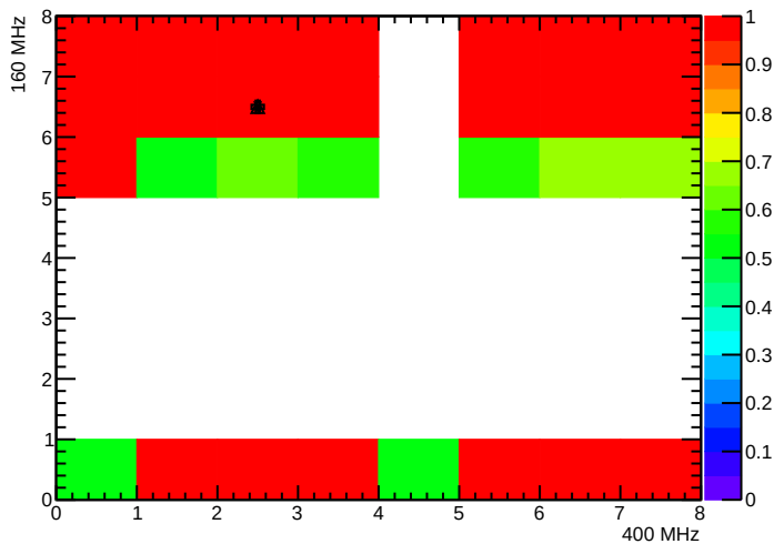
BPix_BmO_SEC3_LYR2_LDR5F_MOD1_nTBMDecodes
