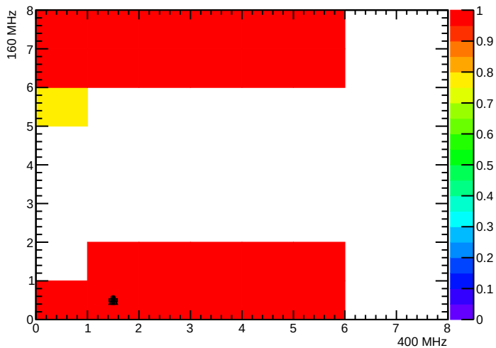
BPix_BpO_SEC1_LYR4_LDR2F_MOD4_nTBMDecodes
