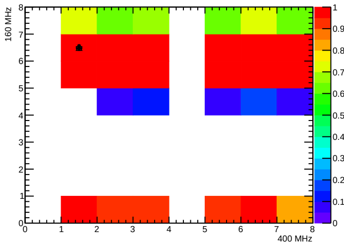
BPix_Bml_SEC6_LYR1_LDR5H_MOD4_nTBMDecodes
