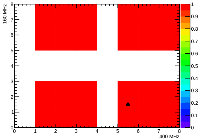
BPix_BpI_SEC3_LYR2_LDR5F_MOD3_nTBMDecodes
