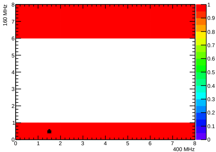
BPix_BpO_SEC6_LYR3_LDR16F_MOD3_nTBMDecodes
