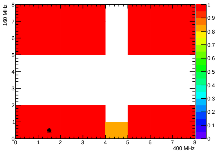
BPix_Bml_SEC8_LYR2_LDR13F_MOD2_nTBMDecodes
