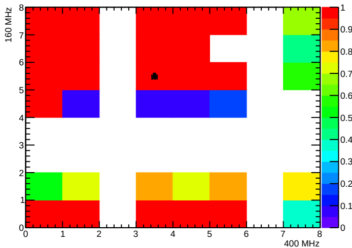
BPix_Bml_SEC8_LYR1_LDR6H_MOD2_nTBMDecodes
