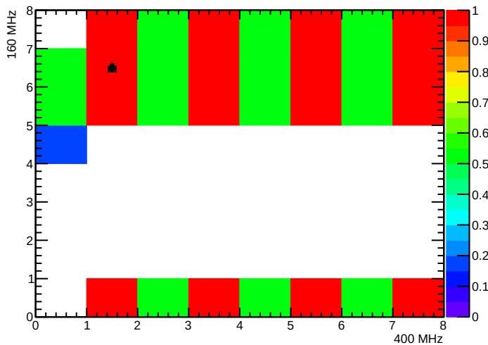
BPix_BpO_SEC7_LYR1_LDR5H_MOD1_nTBMDecodes
