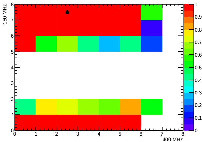
BPix_Bpl_SEC6_LYR2_LDR10F_MOD2_nTBMDecodes
