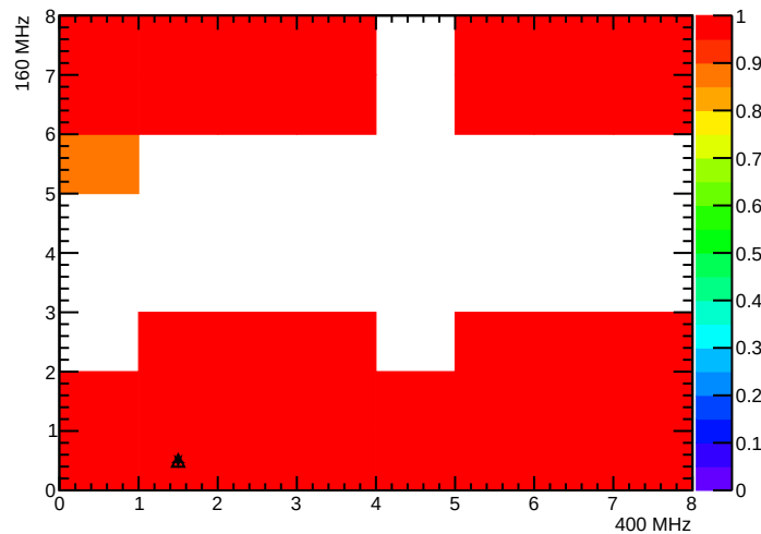
BPix_Bml_SEC2_LYR3_LDR5F_MOD4_nROCHheaders
