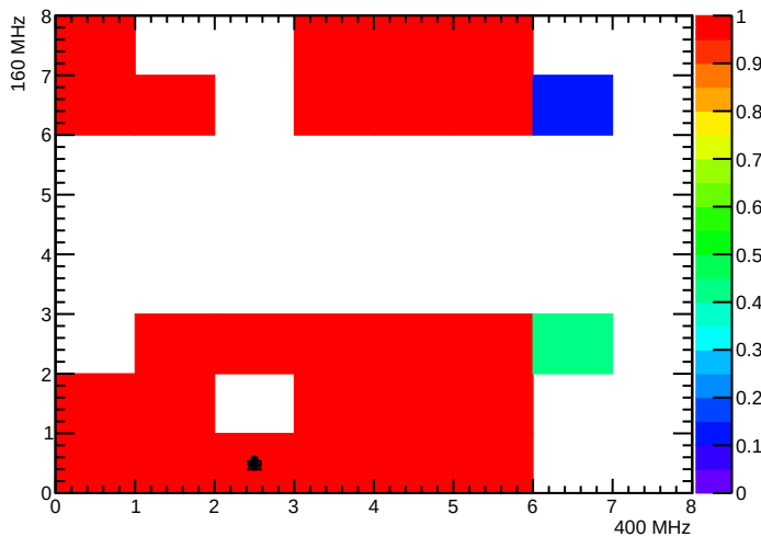
BPix_Bml_SEC2_LYR4_LDR7F_MOD2_nTBMDecodes
