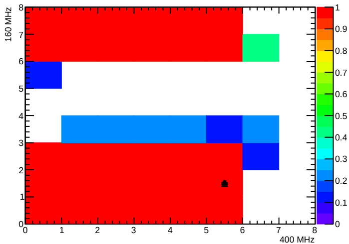
BPix_BpI_SEC1_LYR3_LDR2F_MOD4_nTBMDecodes
