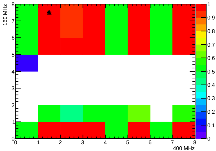
BPix_BpI_SEC2_LYR1_LDR1H_MOD1_nTBMDecodes
