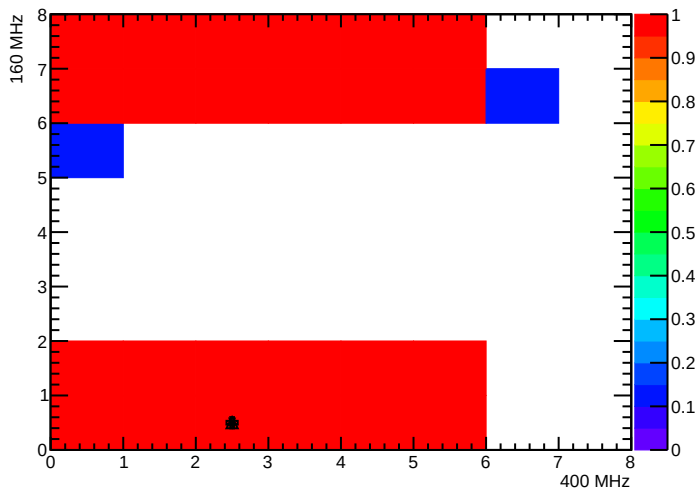
BPix_BpO_SEC8_LYR4_LDR31F_MOD4_nTBMDecodes
