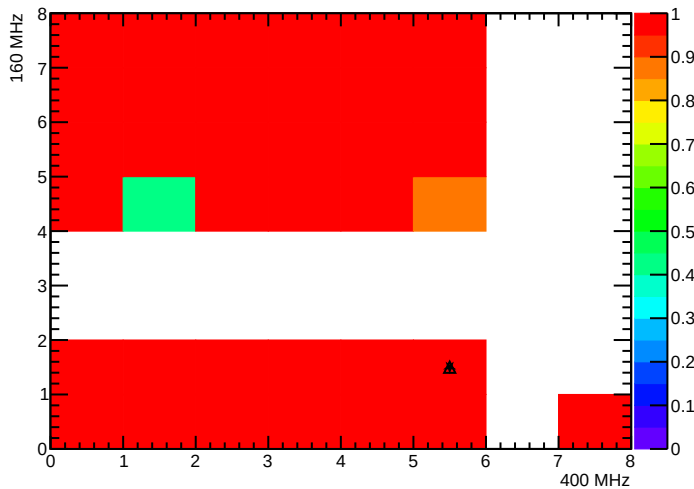
BPix_BpO_SEC4_LYR2_LDR7F_MOD2_nROCHheaders
