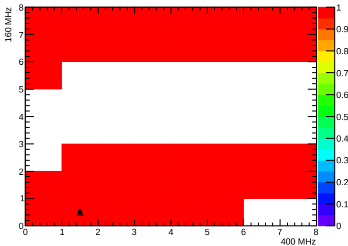
BPix_BmO_SEC1_LYR3_LDR2F_MOD2_nROCHheaders
