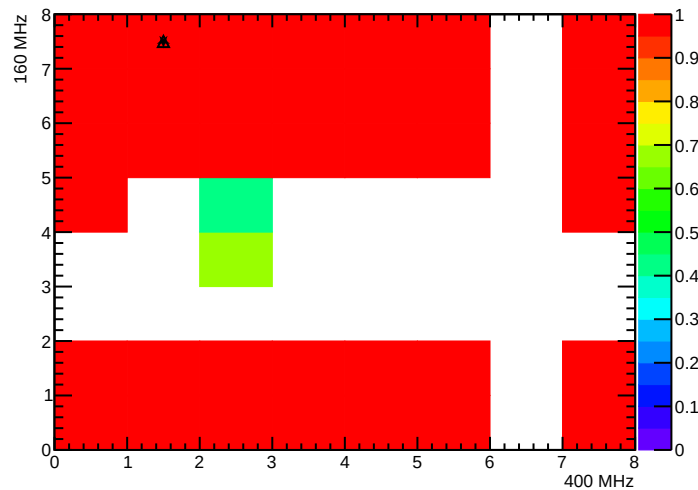
BPix_Bml_SEC4_LYR1_LDR3H_MOD2_nROCHheaders
