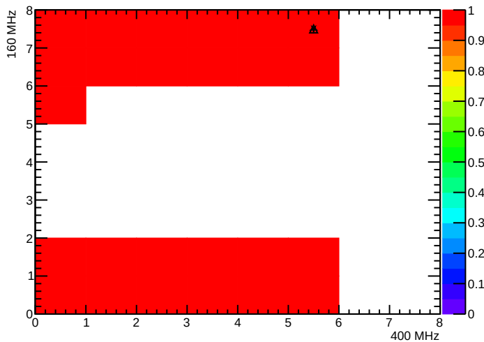
BPix_BmO_SEC2_LYR3_LDR5F_MOD2_nROCHheaders
