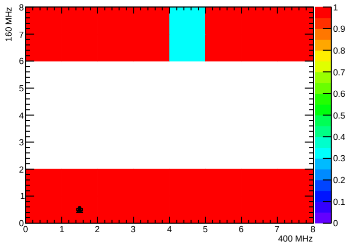
BPix_BmO_SEC5_LYR3_LDR13F_MOD4_nTBMDecodes
