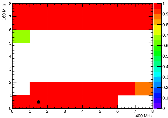
BPix_Bml_SEC1_LYR4_LDR4F_MOD2_nTBMDecodes
