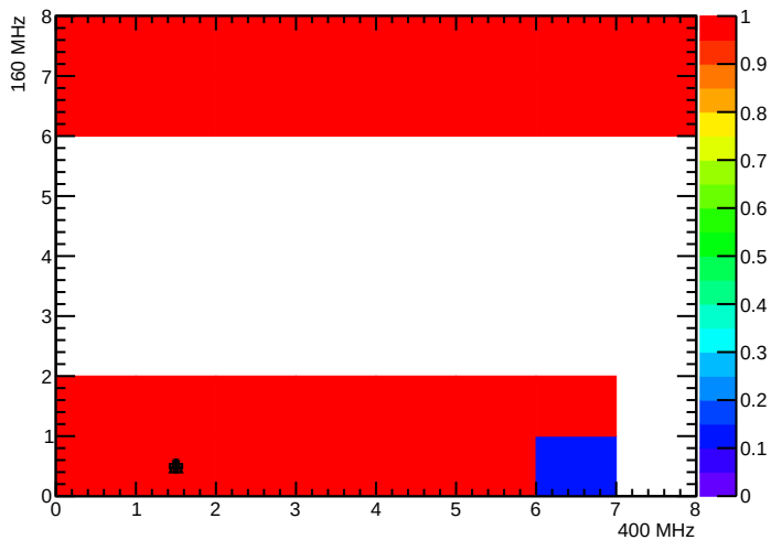
BPix_Bpl_SEC8_LYR4_LDR31F_MOD3_nTBMDecodes
