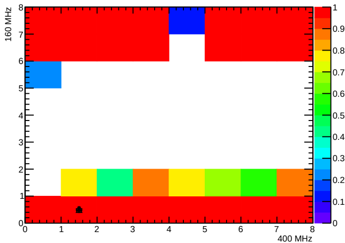
BPix_Bml_SEC3_LYR3_LDR6F_MOD4_nTBMDecodes
