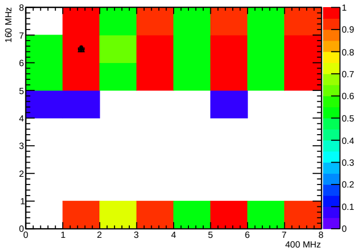
BPix_BpI_SEC6_LYR1_LDR5H_MOD4_nTBMDecodes
