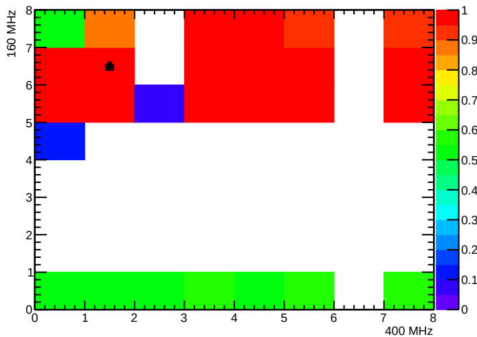
BPix_BpO_SEC6_LYR1_LDR5H_MOD3_nTBMDecodes
