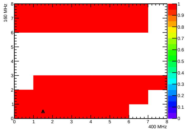
BPix_BmO_SEC8_LYR4_LDR32F_MOD3_nROCHheaders
