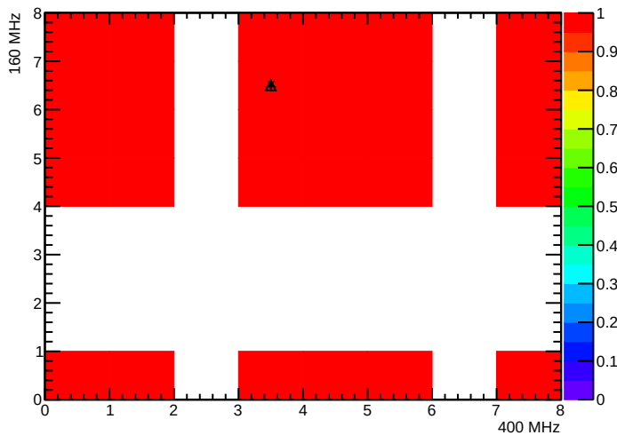
BPix_BmO_SEC4_LYR1_LDR3H_MOD3_nROCHheaders
