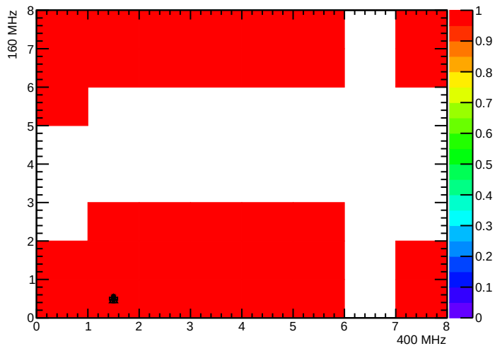
BPix_BpO_SEC5_LYR4_LDR20F_MOD1_nTBMDecodes
