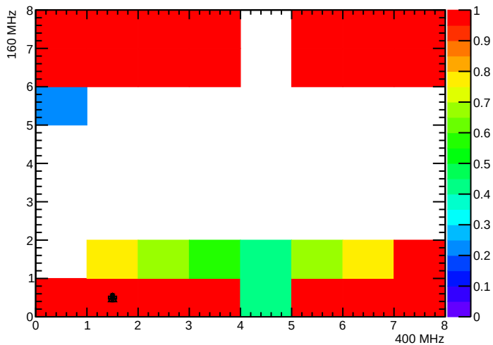
BPix_Bpl_SEC8_LYR3_LDR22F_MOD4_nTBMDecodes
