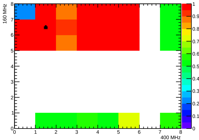
BPix_BpO_SEC7_LYR1_LDR5H_MOD2_nTBMDecodes
