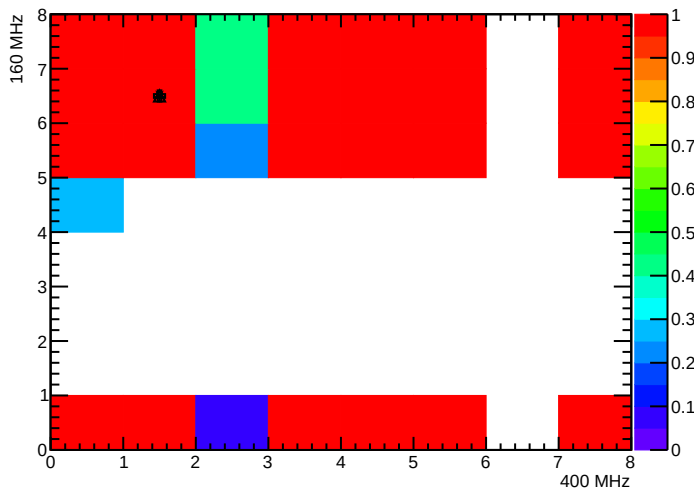
BPix_BpO_SEC3_LYR1_LDR2F_MOD2_nTBMDecodes
