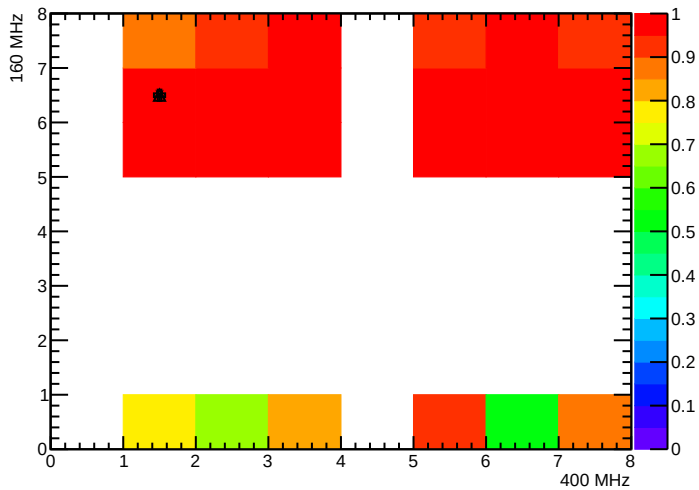
Bpix_Bpl_SEC7_LYR1_LDR5H_MOD2_nTBMDecodes
