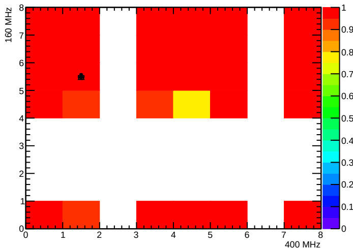
BPix_BmO_SEC6_LYR1_LDR5F_MOD3_nTBMDecodes
