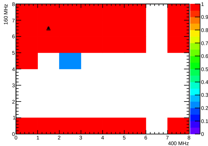
BPix_BpI_SEC4_LYR1_LDR3H_MOD1_nROCHheaders
