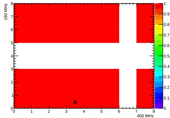
BPix_BmO_SEC8_LYR2_LDR13F_MOD4_nROCHheaders
