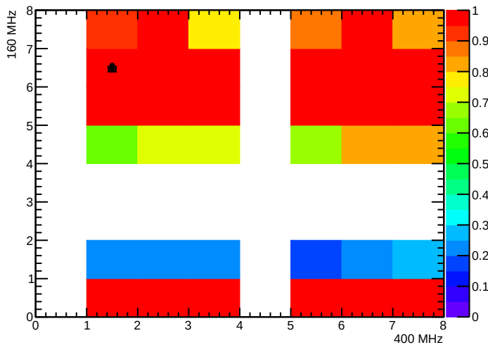
BPix_BpO_SEC8_LYR1_LDR6F_MOD3_nTBMDecodes
