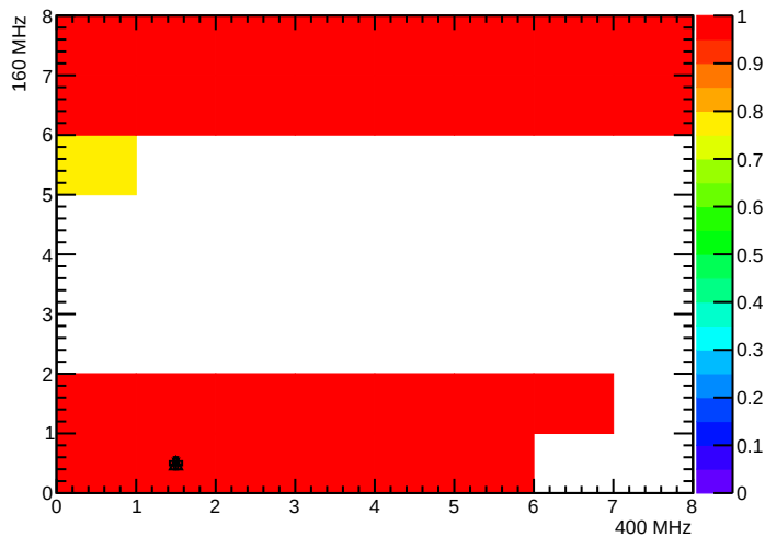
BPix_BmO_SEC7_LYR3_LDR18F_MOD3_nTBMDecodes
