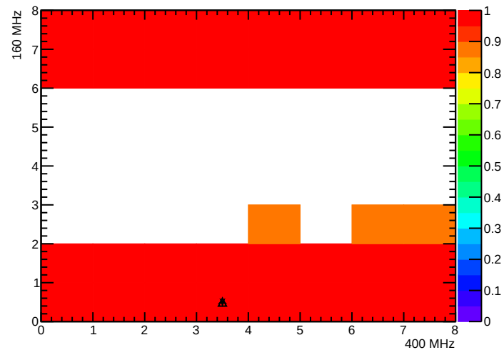
BPix_BpO_SEC4_LYR4_LDR15F_MOD1_nROCHheaders
