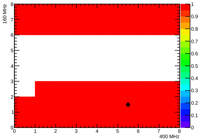
BPix_BpI_SEC1_LYR4_LDR1F_MOD4_nTBMDecodes
