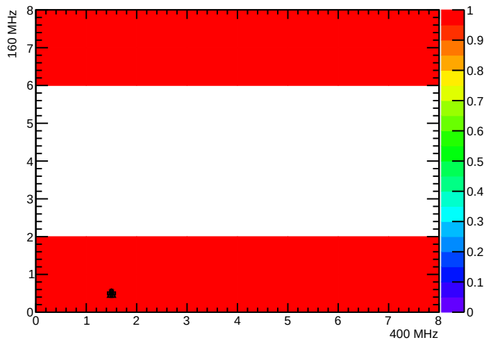
BPix_BmO_SEC7_LYR3_LDR20F_MOD3_nTBMDecodes
