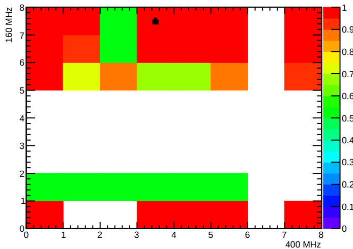
BPix_BpO_SEC7_LYR2_LDR11F_MOD2_nTBMDecodes
