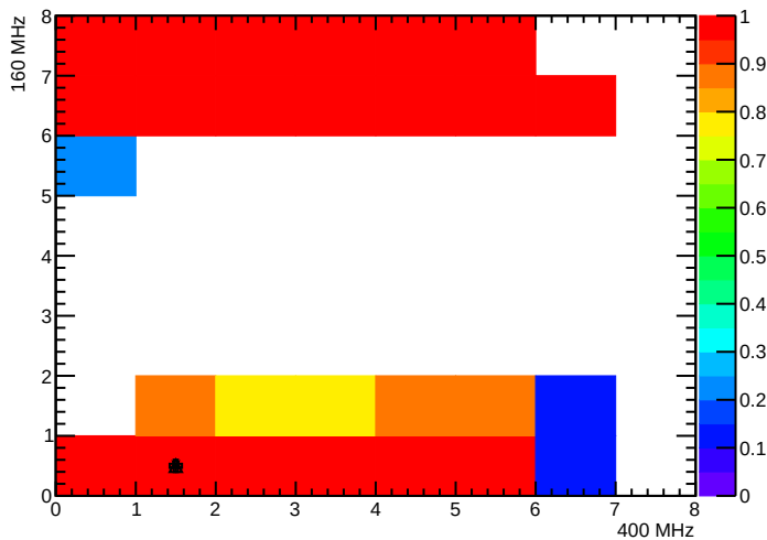
BPix_BpO_SEC3_LYR3_LDR6F_MOD4_nTBMDecodes
