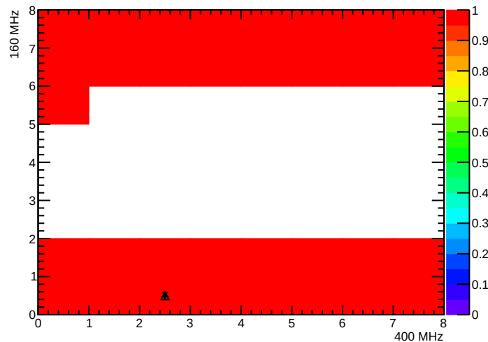
BPix_Bml_SEC8_LYR4_LDR31F_MOD1_nROCHheaders
