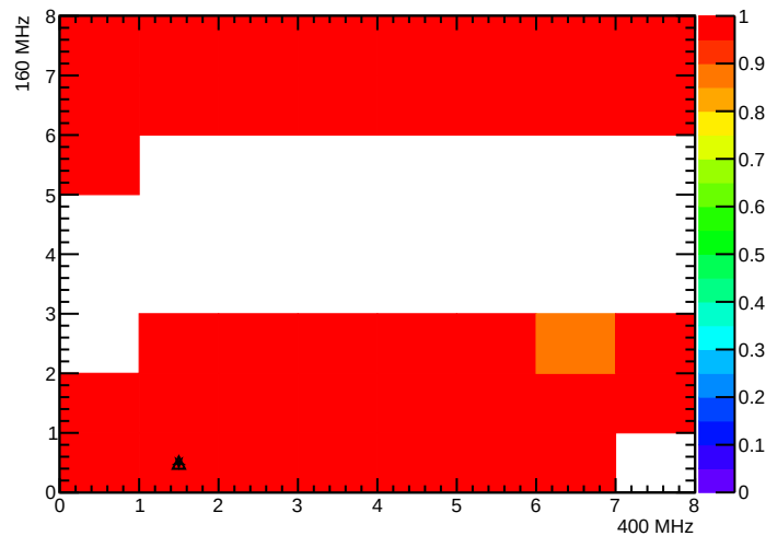
BPix_BmO_SEC6_LYR3_LDR16F_MOD3_nROCHheaders
