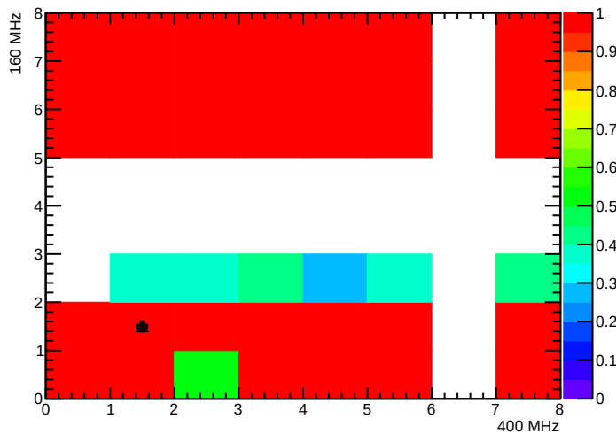
BPix_BmO_SEC7_LYR2_LDR12F_MOD2_nTBMDecodes
