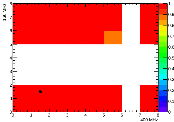
BPix_BmO_SEC7_LYR2_LDR12F_MOD1_nTBMDecodes
