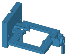
P07 Camera cradle
