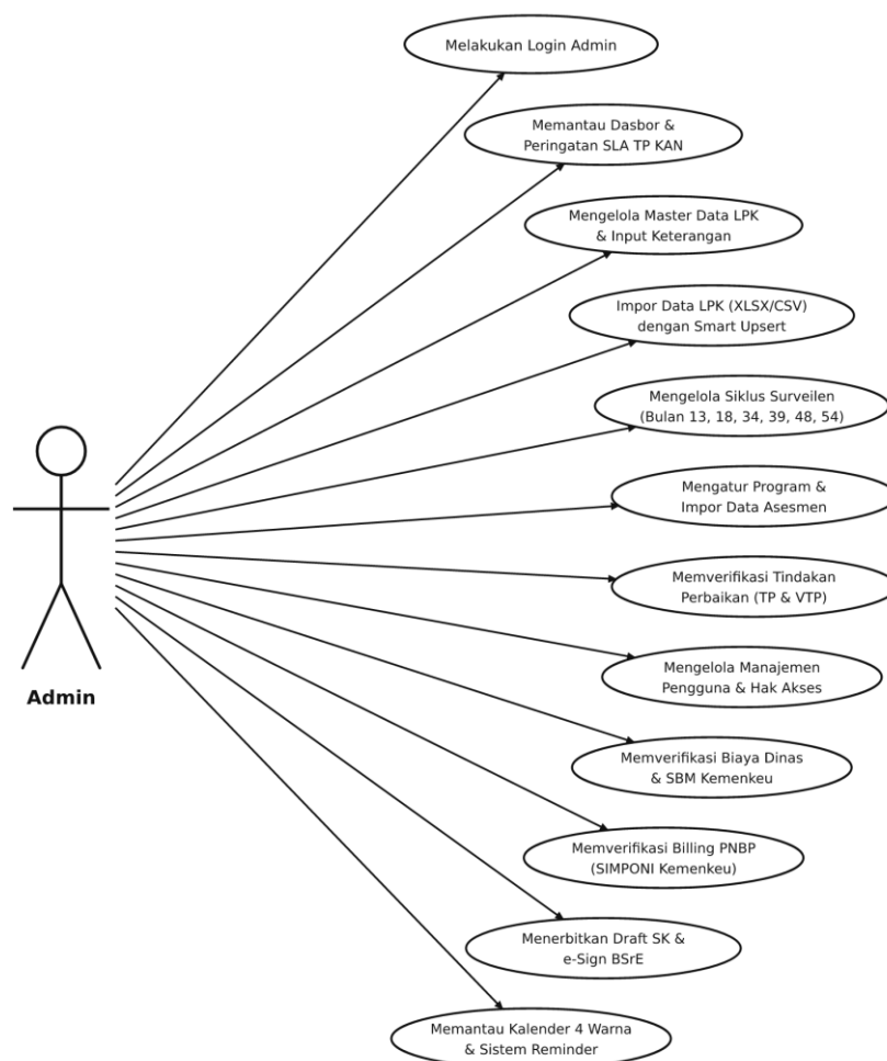
Gambar 2. 3 Use Case Diagram Administrator Unit Akreditasi
