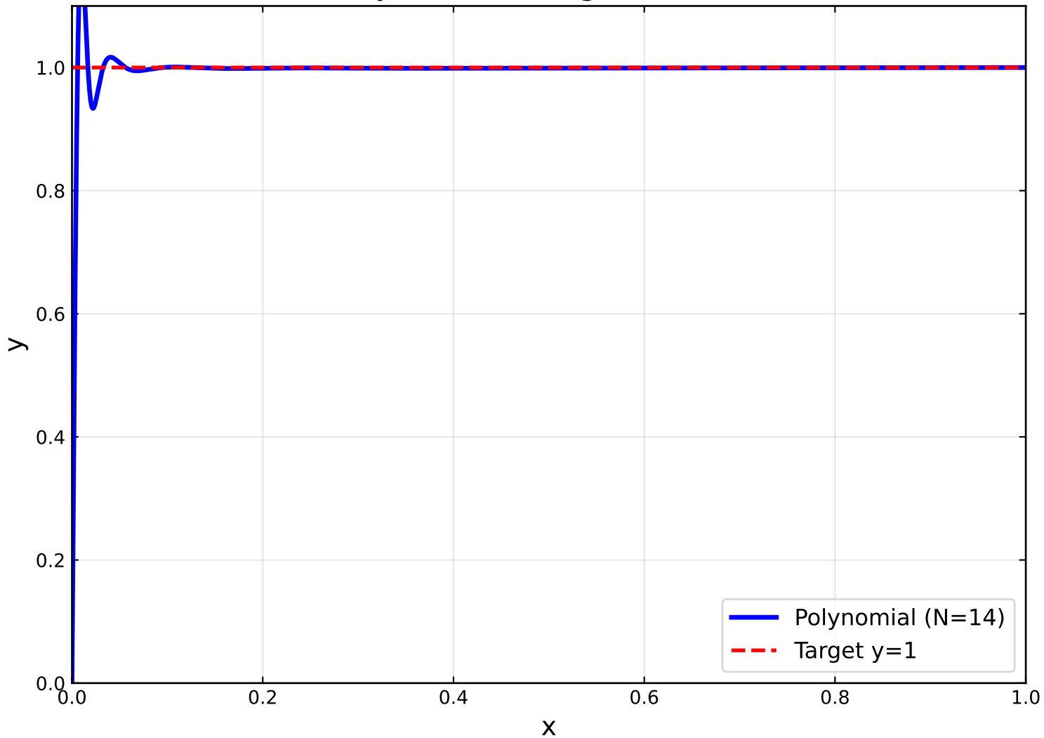
Polynomial Fitting with N=14
