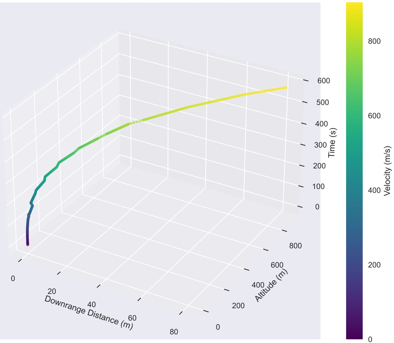
3D Rocket Trajectory (Colored by Velocity)
