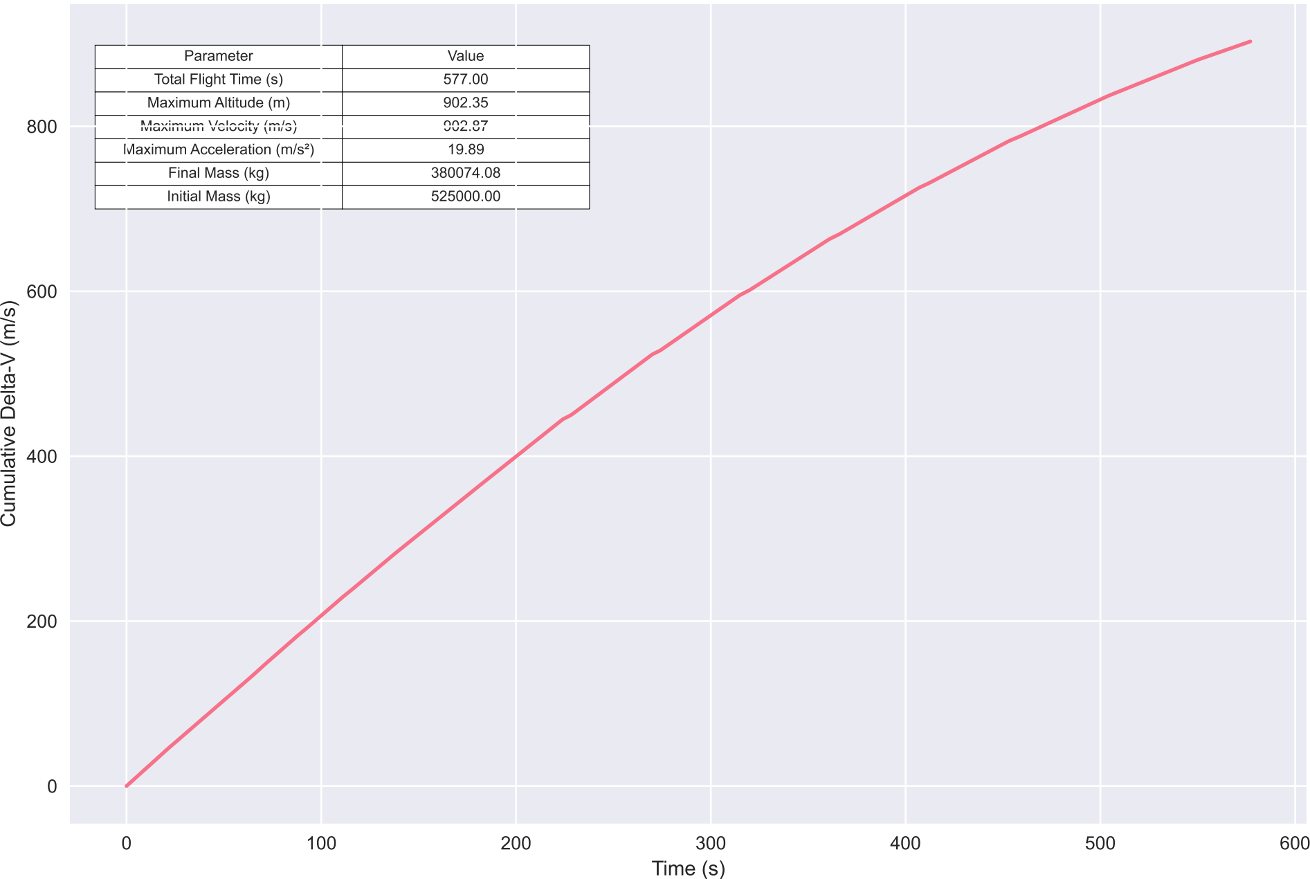
Cumulative Delta-V vs Time
