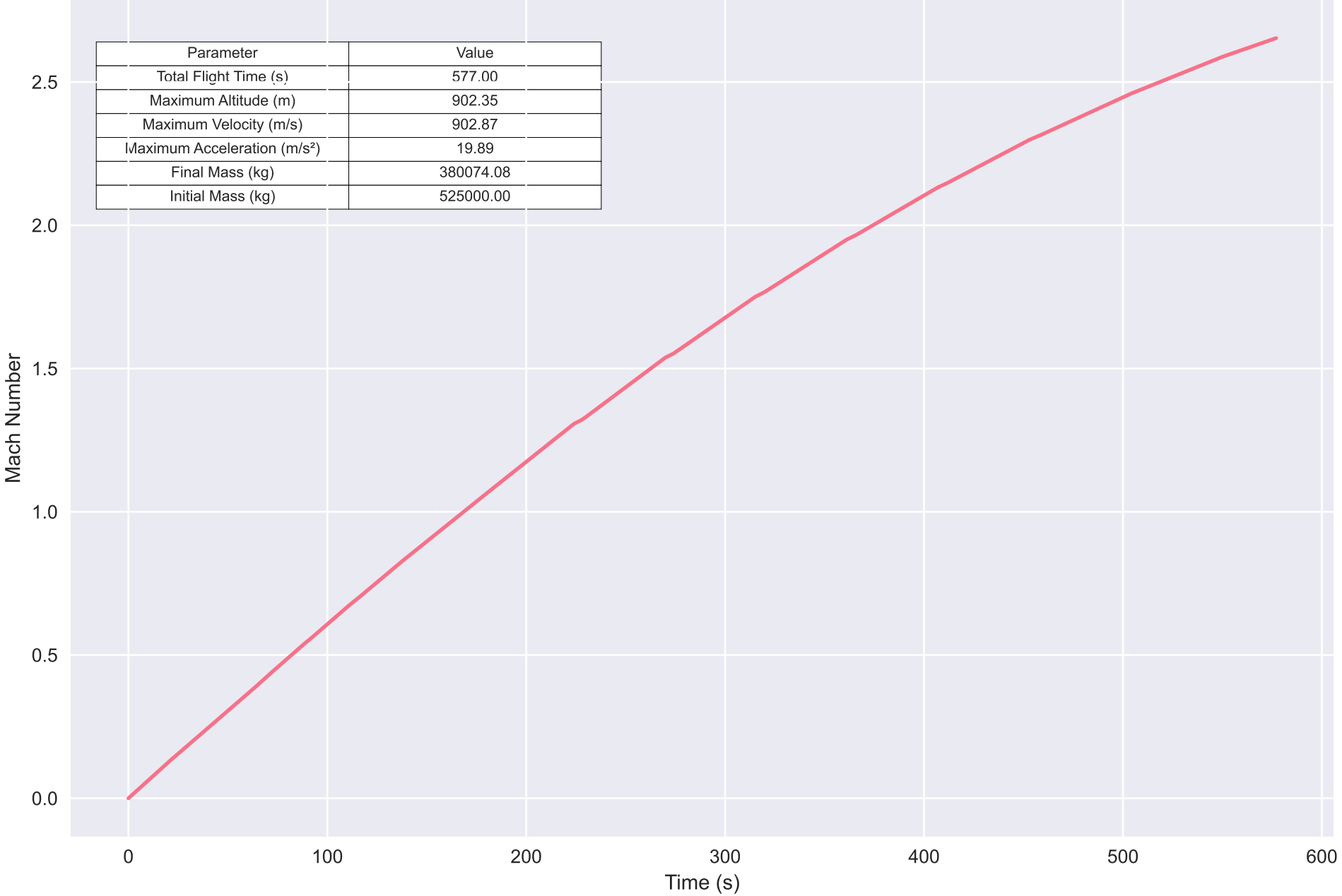
Mach Number vs Time
