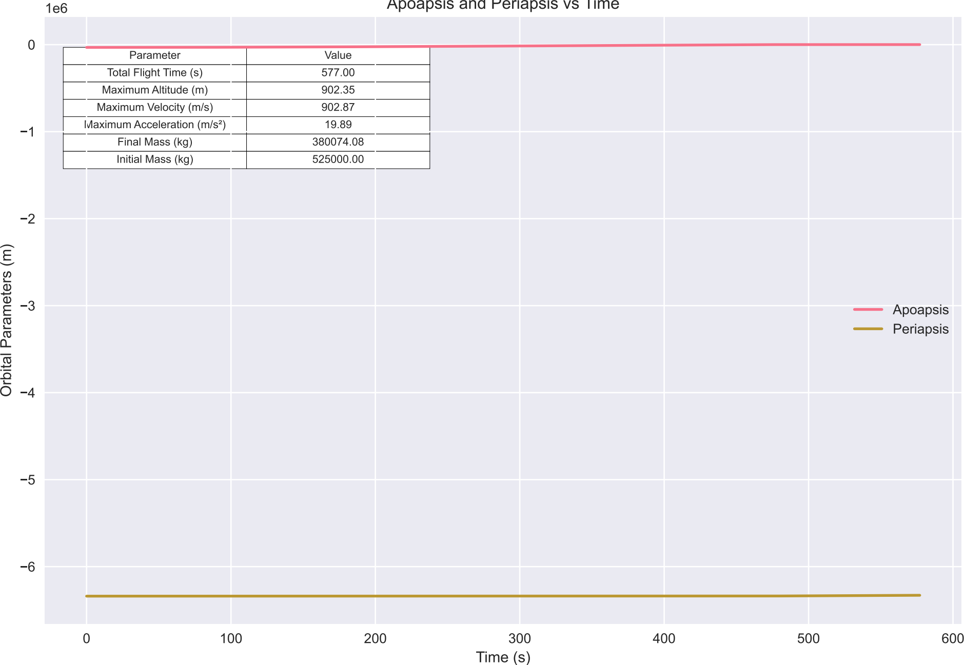
Apoapsis and Periapsis vs Time
