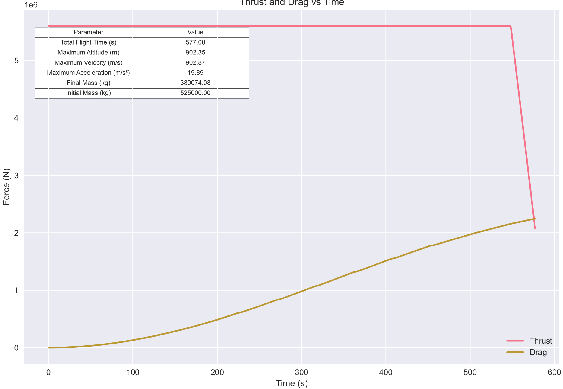
Thrust and Drag vs Time
