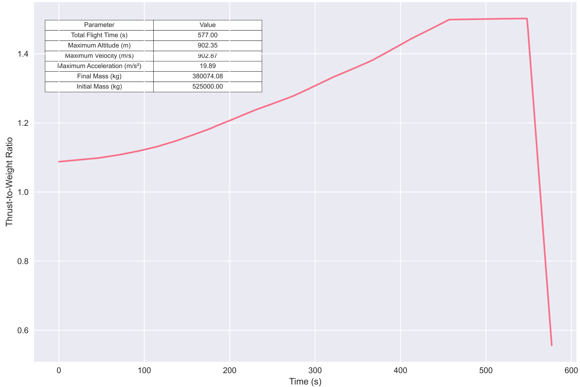
Thrust-to-Weight Ratio vs Time
