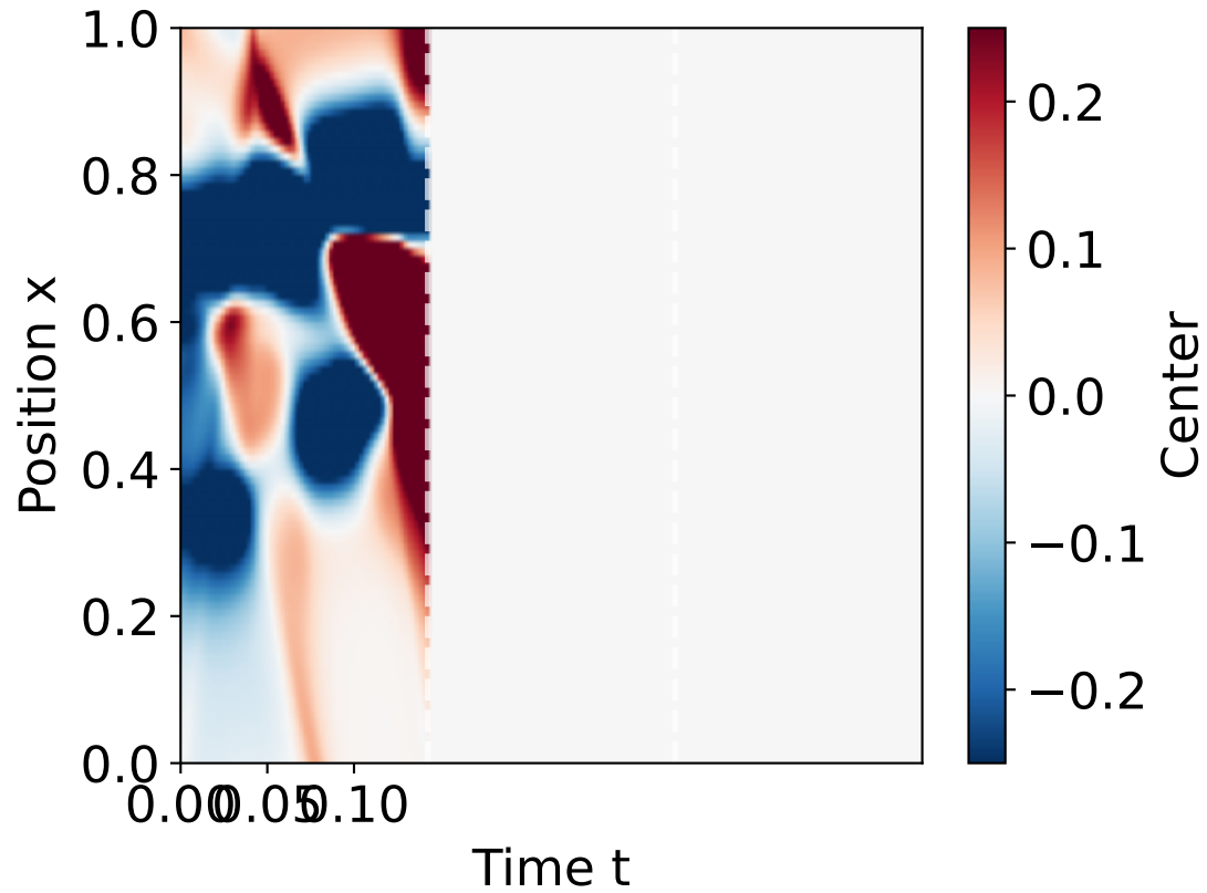
VI Mean Prediction
