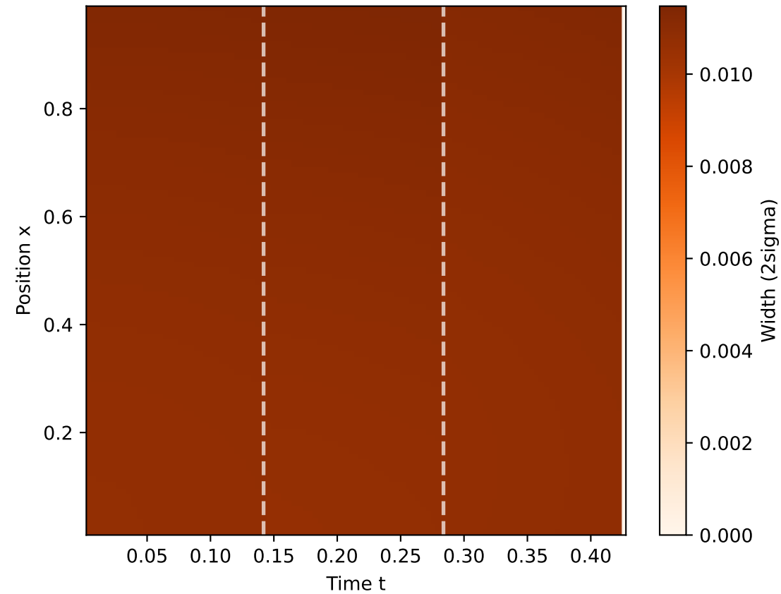
VI (coeff) Uncertainty (95% CI Width)
