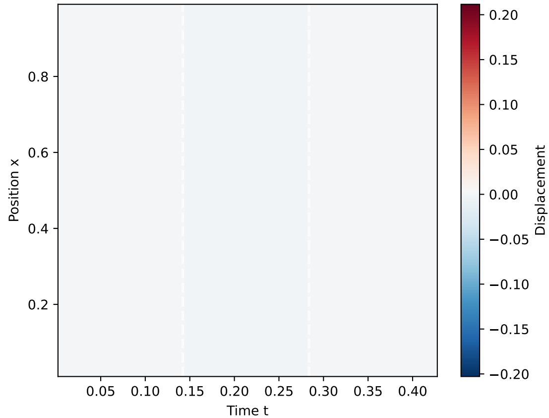
VI (coeff) Mean Prediction
