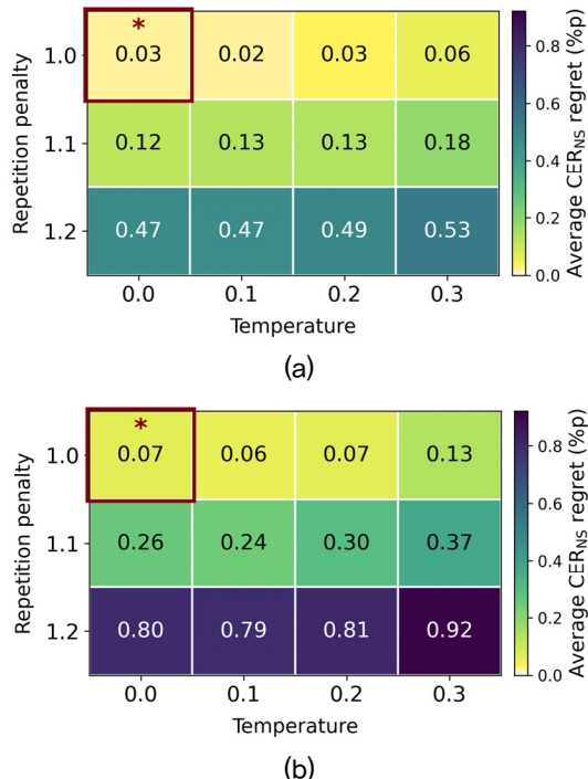
Fig. 2. (Color available online) Average CER NS regret (%) across the ten evaluation sets by temperature and repetition penalty (language = korean, max_new_tokens = 512): (a) 1.7B, (b) 0.6B. The asterisk marks the recommended setting.
