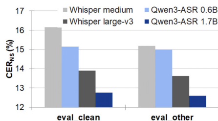
Fig. 3. (Color available online) CER NS of Qwen3-ASR and Whisper on KsponSpeech eval_clean and eval_other. Models are paired by comparable scale (1.7B and large-v3; 0.6B and medium), and each uses its best decoding setting on these sets. Lower is better.
