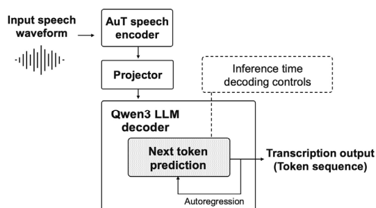
Fig. 1. Architecture of Qwen3-ASR and the decoding stage where inference settings act.
