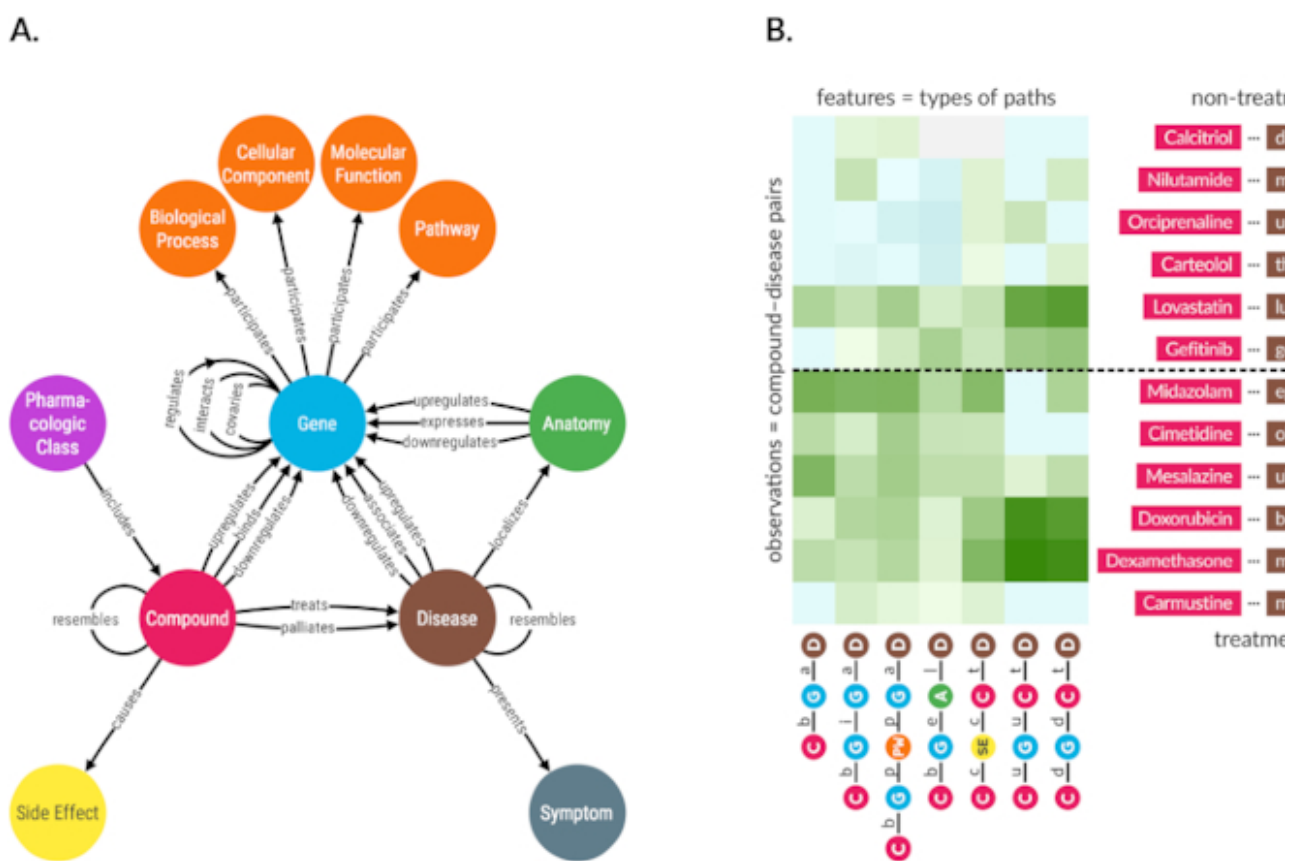
Figure 1: A- (A) Hetionet v1.0 metagraph. The types of nodes and edges in Hetionet.
