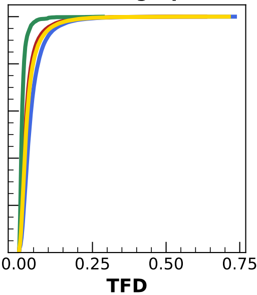
Torsion Fingerprints
