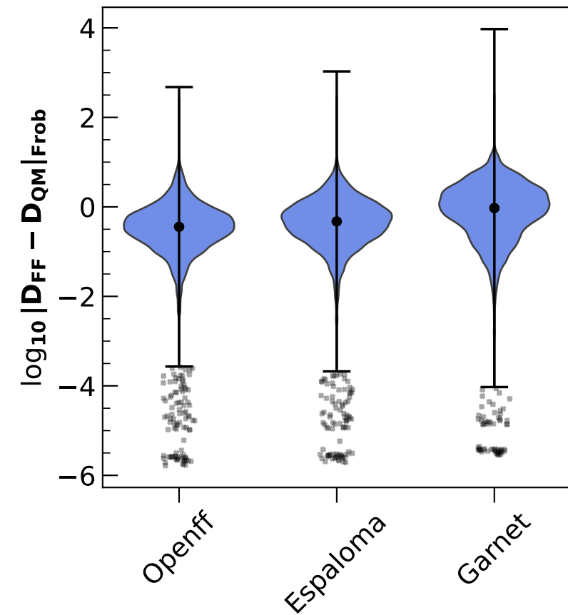
Frobenius Difference
