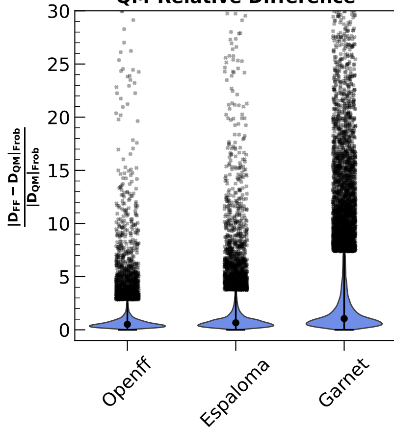
QM-Relative Difference
